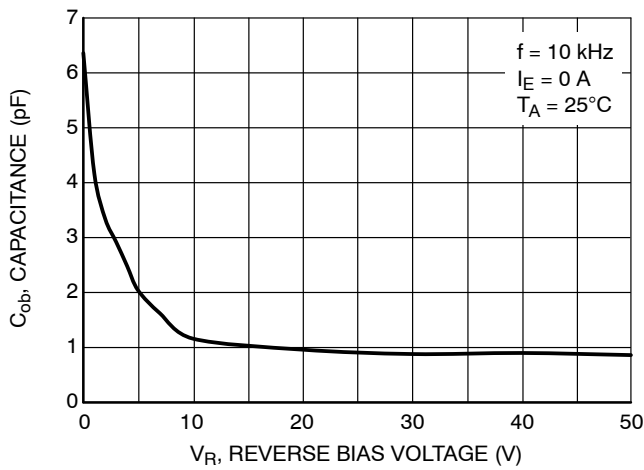
Figure 19. Output Capacitance
