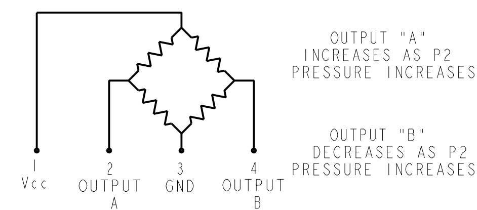
CIRCUIT DIAGRAM
