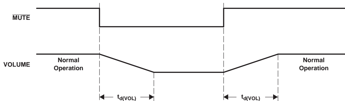
Figure 3-8. Mute Timing
