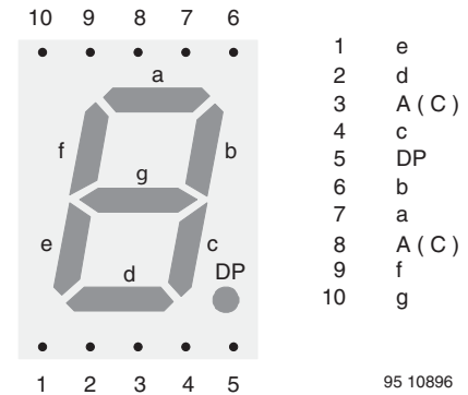
Fig. 7 - TDSR1350/1360
