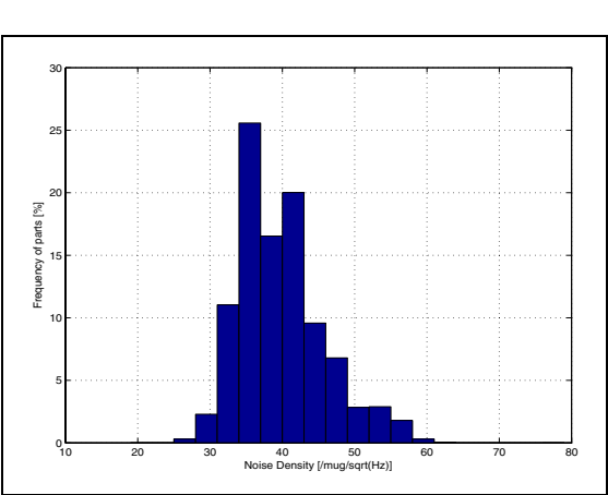
Figure 20. Noise density at 3.3 V (Z axis)
