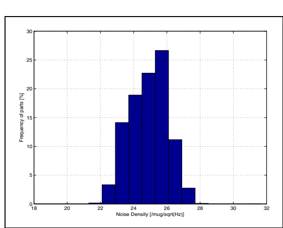
Figure 19. Noise density at 3.3 V (X, Y axis)
