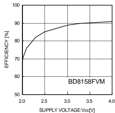
Fig. 13 Power Efficiency vs Power Supply Voltage
