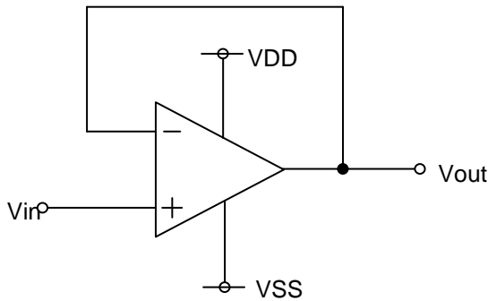
Fig.146 Voltage follower
