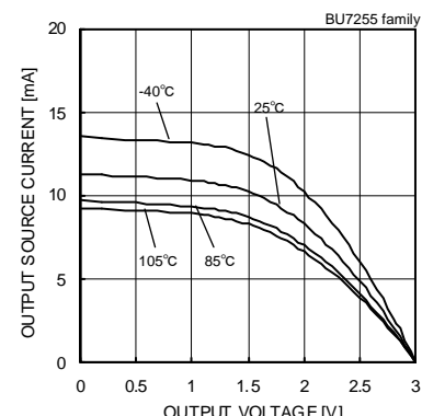
Fig.32 Output Source Current - Output Voltage (VDD=3[V])
