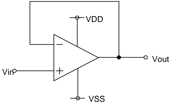
Fig.146 Voltage follower
