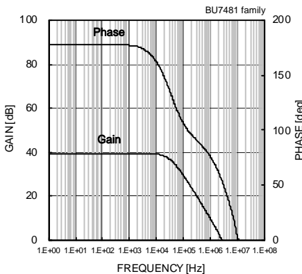
Fig.92 Voltage Gain – Frequency
