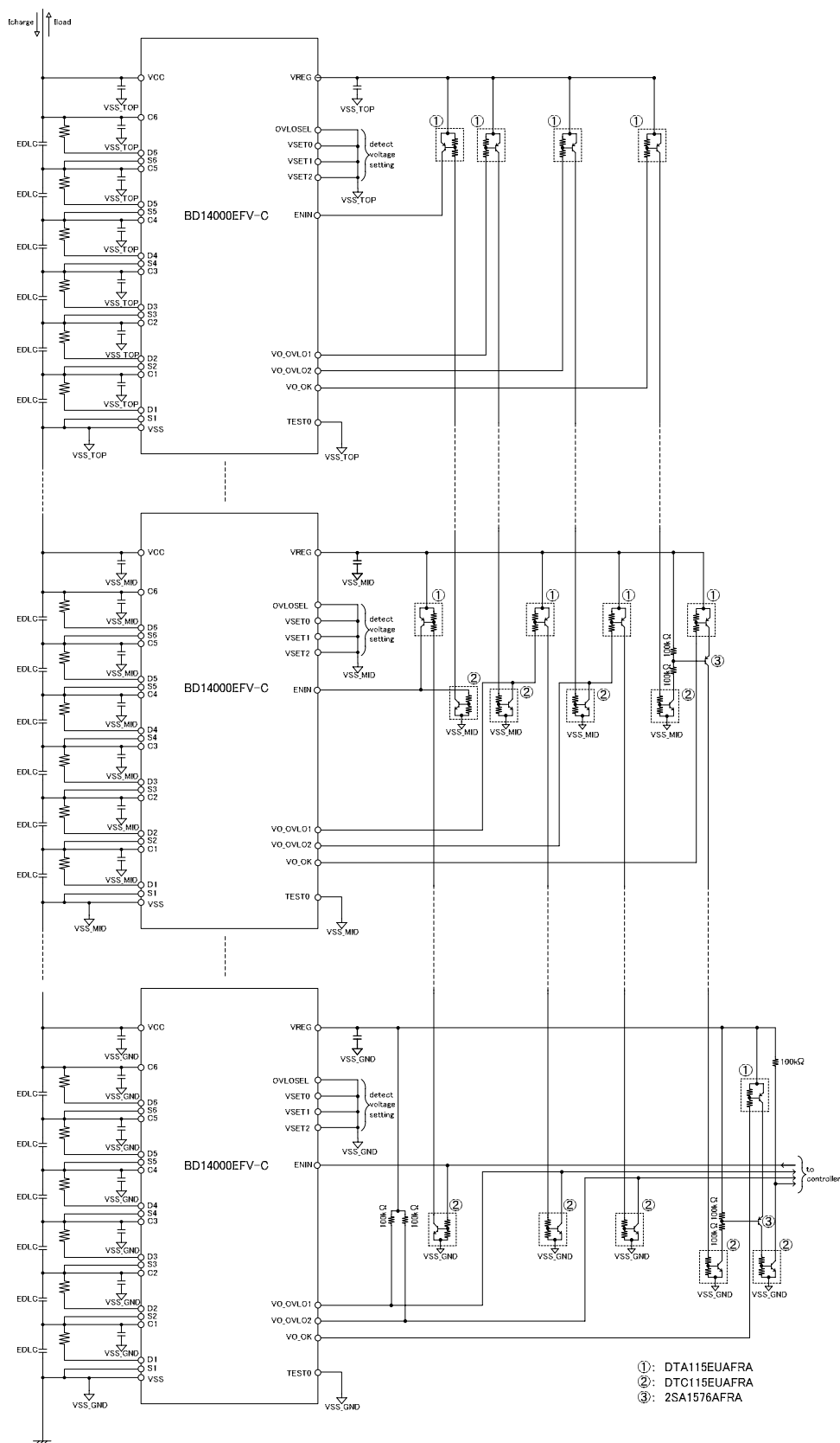
Figure 10. Application circuit for BD14000EFV-C series connection
