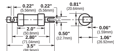
CGL 40-50
