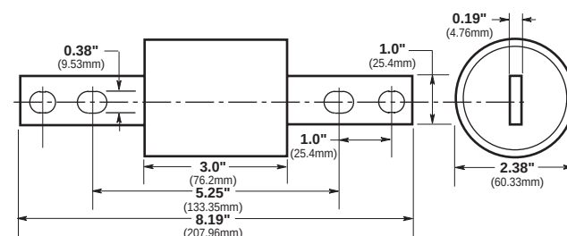
CGL 225-400
