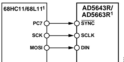
Figure 57. AD5623R/AD5643R/AD5663R to 68HC11/68L11 Interface
