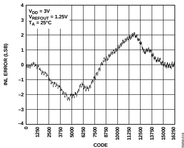
Figure 17. INL—AD5643R-3
