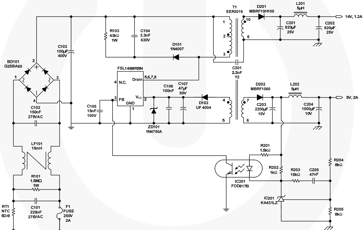
Figure 25. Schematic
