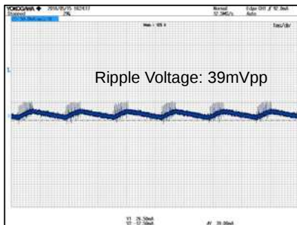
Figure 18. VOUT Ripple Voltage.1 V_{IN}=100\text{Vac} , I_{OUT}=10\text{mA} CH1: VOUT 50mV/div, 1000 \mu\text{s} /div
