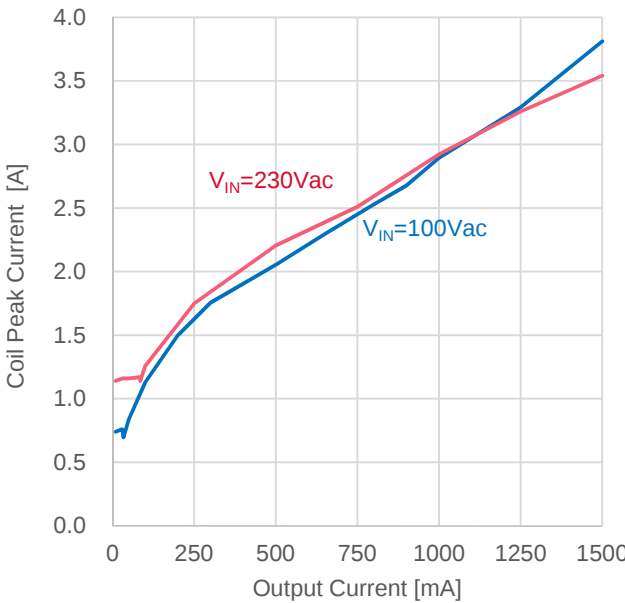
Figure 16. Secondary Peak Current ( I_{OUT} vs. I_{peak} )
