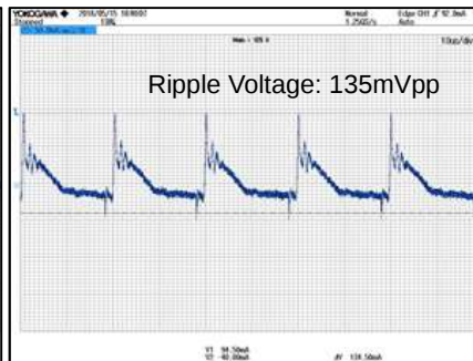
Figure 22. VOUT Ripple Voltage.5 V_{IN}=230\text{Vac} , I_{OUT}=500\text{mA} CH1: VOUT 50mV/div, 10 \mu\text{s} /div
