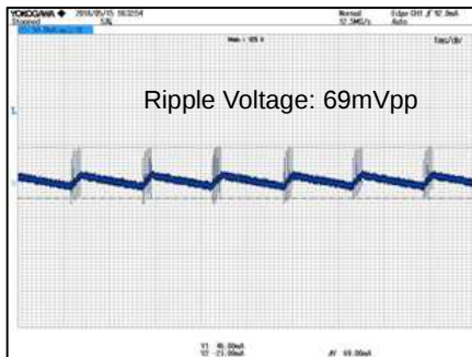
Figure 21. VOUT Ripple Voltage.4 V_{IN}=230\text{Vac} , I_{OUT}=10\text{mA} CH1: VOUT 50mV/div, 1000 \mu\text{s} /div
