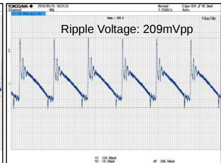
Figure 23. VOUT Ripple Voltage.6 V_{IN}=230\text{Vac} , I_{OUT}=1500\text{mA} CH1: VOUT 50mV/div, 10 \mu\text{s} /div
