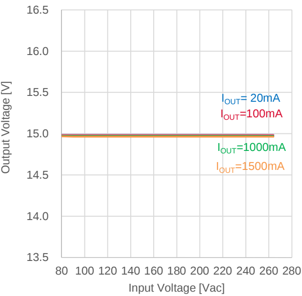
Figure 12. LINE Regulation ( I_{OUT} vs. V_{OUT} )
