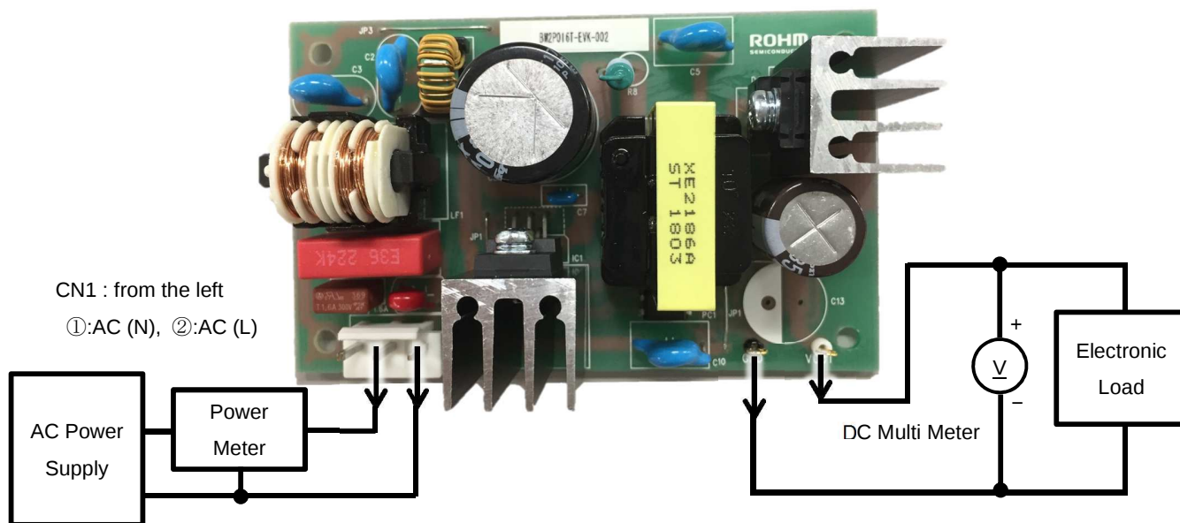
Figure 1. Connection Circuit
