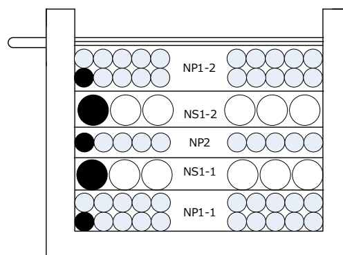
Figure 7. Winding structure diagram
