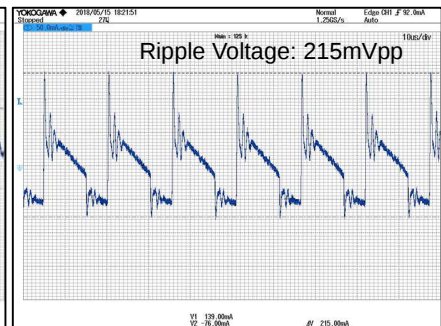
Figure 20. VOUT Ripple Voltage.3 V_{IN}=100\text{Vac} , I_{OUT}=1500\text{mA} CH1: VOUT 50mV/div, 10 \mu\text{s} /div
