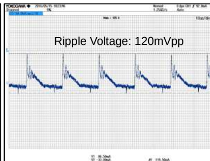
Figure 19. VOUT Ripple Voltage.2 V_{IN}=100\text{Vac} , I_{OUT}=500\text{mA} CH1: VOUT 50mV/div, 10 \mu\text{s} /div
