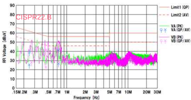
Figure 24. Conducted Emission.1
