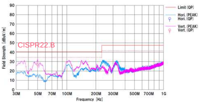
Figure 26. Radiated Emission.1
