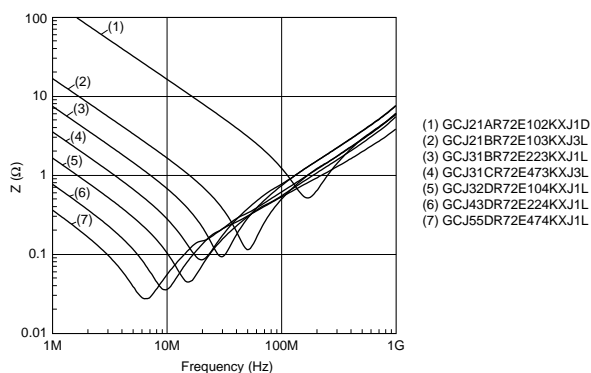
X7R Characteristics DC250V
