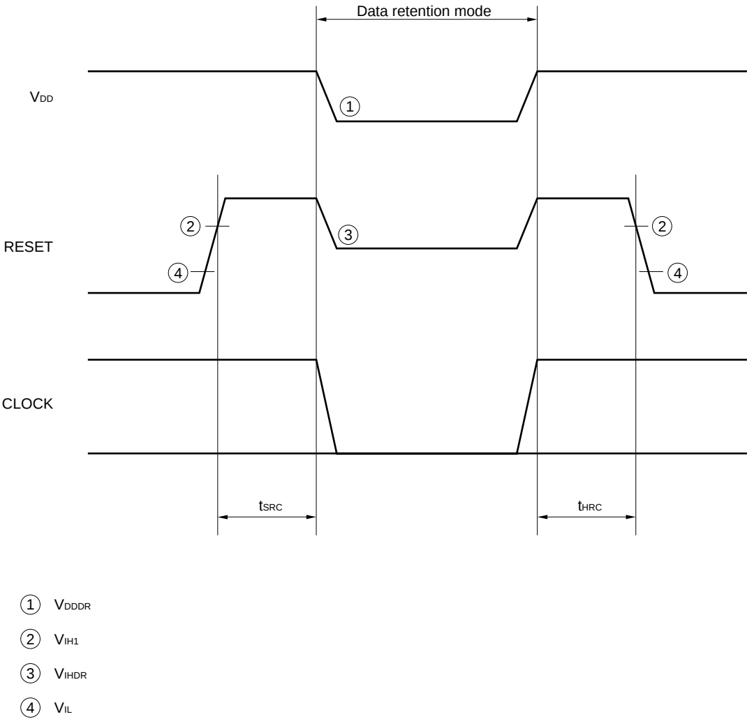
Data retention timing waveforms
