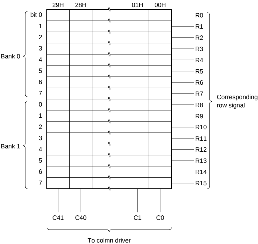
Figure 2-7. Data Memory (16-Time-Division, Single-Chip)
