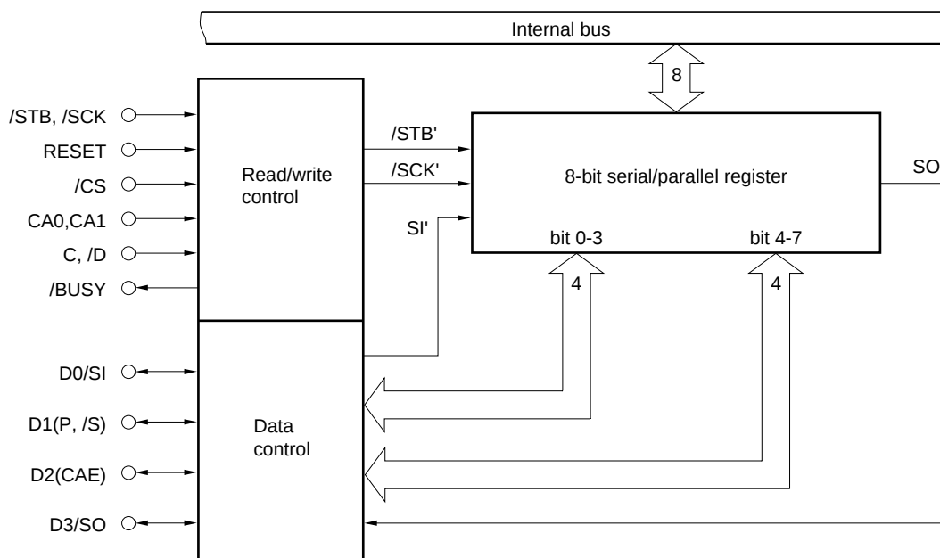
Figure 2-1. Serial/Parallel Interface
