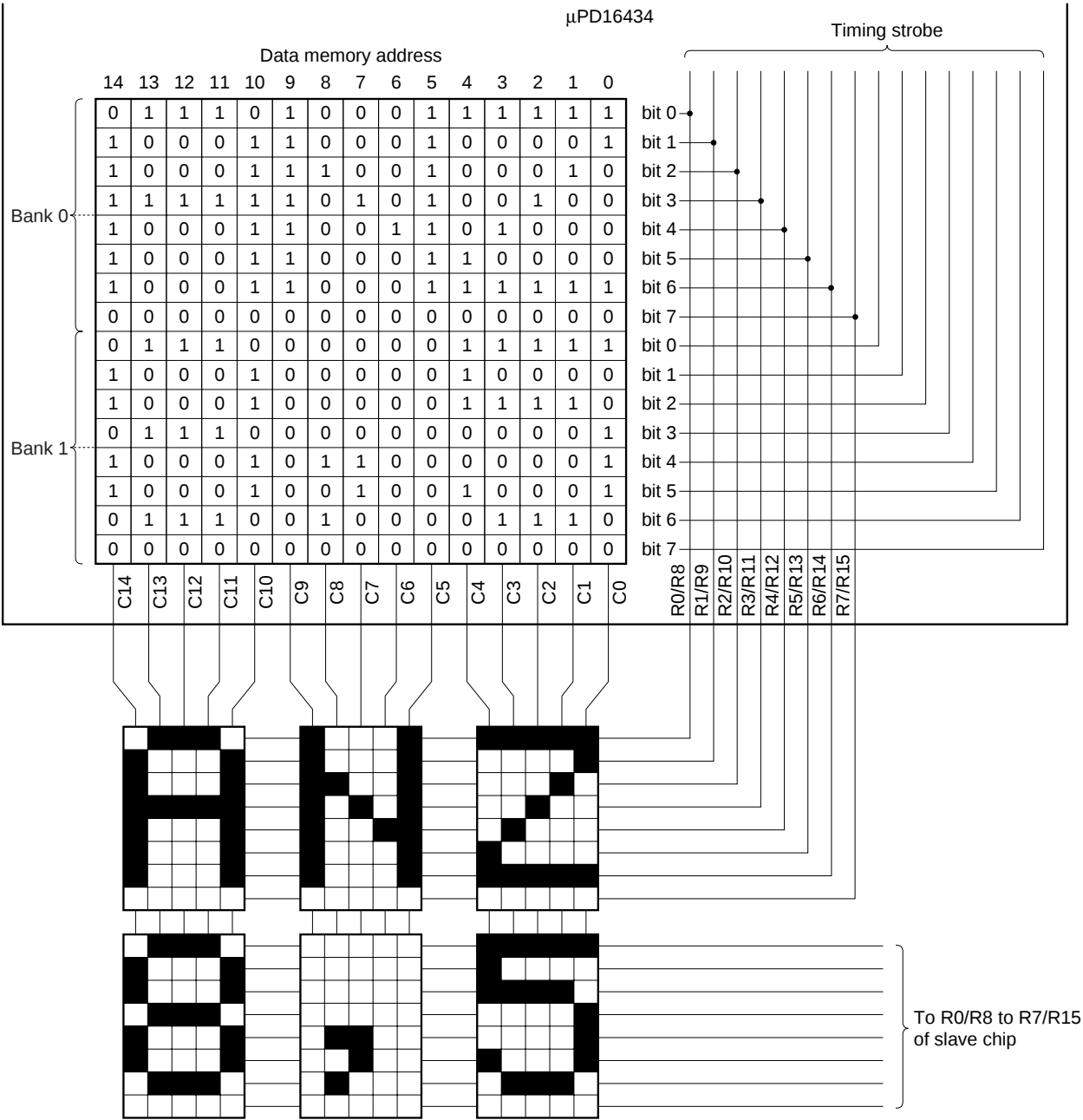
Figure 6-3. 16-Time-divisions
