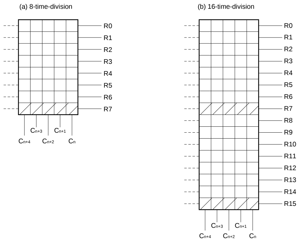
Figure 2-3. LCD Configuration When Using Character Generator
