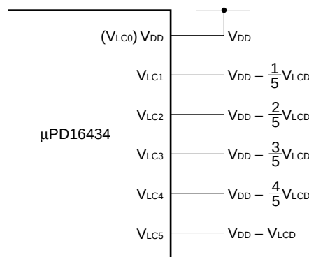
Figure 5–2. 16-Time-Divisions
