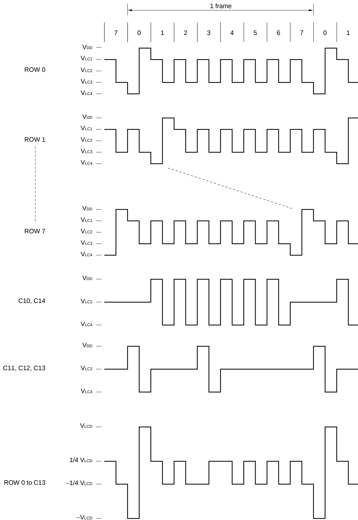
Figure 6–2. 8-Time-divisions (When Displaying Character A)
