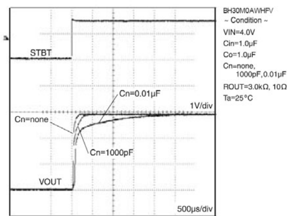
Figure 10. Startup time
