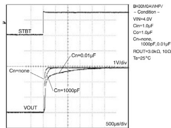
IOUT=300mA (ROUT=10Ω) Figure 10. Startup time
