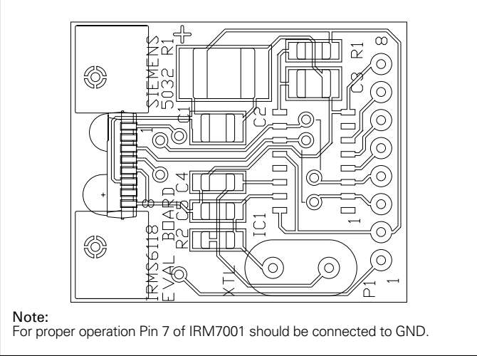
Figure 17. IRMS6118/7001 Eval Board Looking from Back Side
