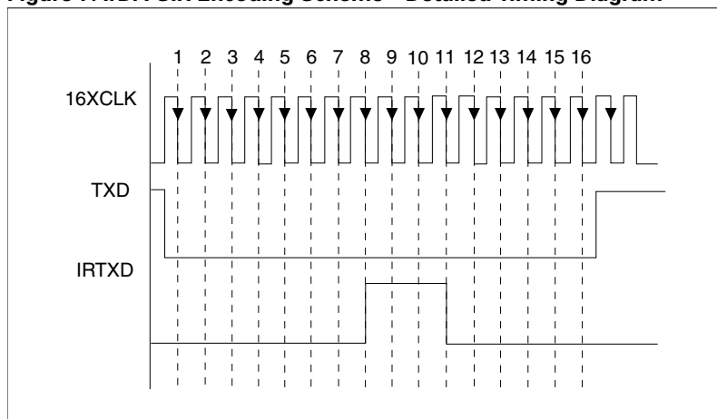
Figure 7. IrDA-SIR Encoding Scheme—Detailed Timing Diagram
