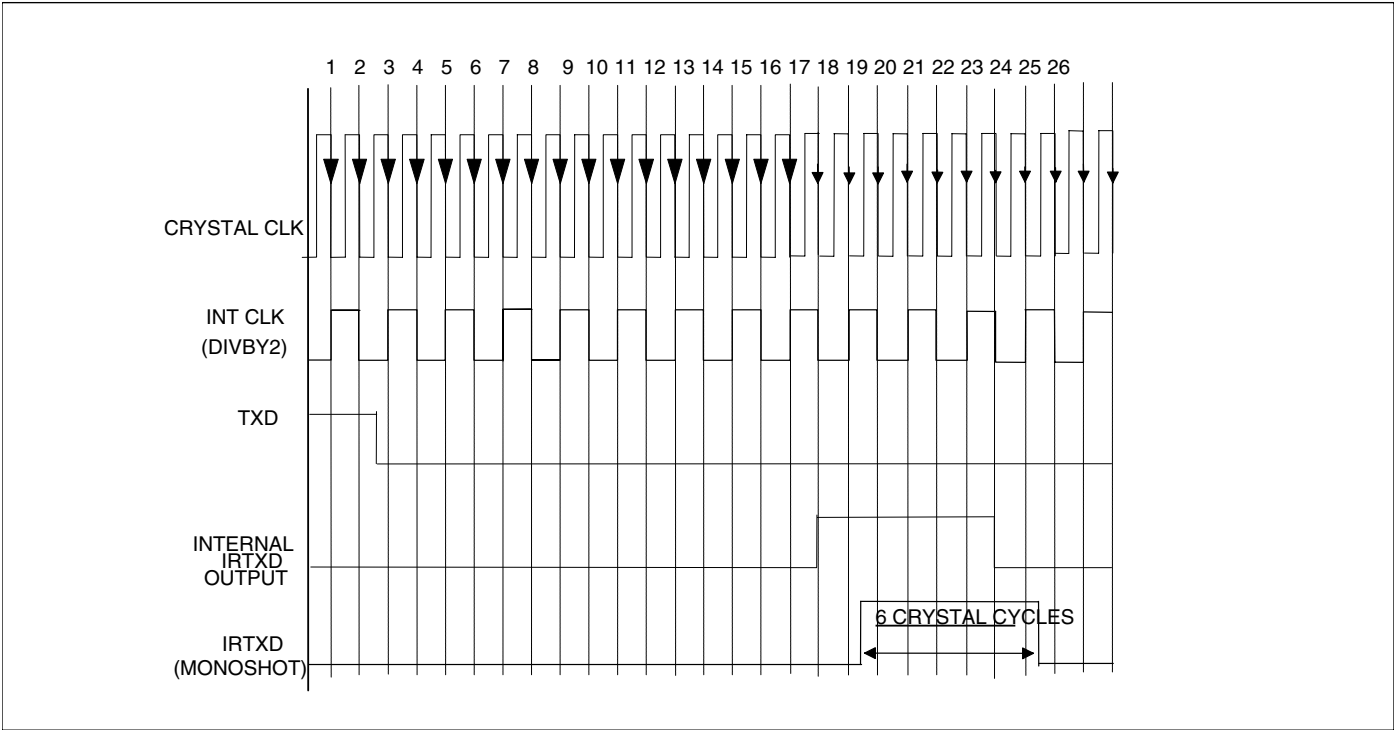
Figure 10. Monoshot Operation
