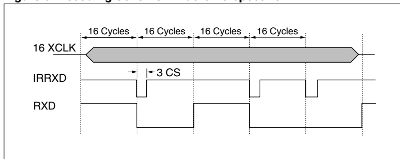
Figure 9. IrDA-SIR Decoding Scheme—Detailed Timing Diagram
