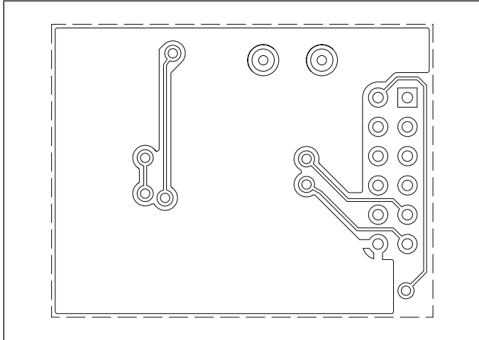
Figure 14. IRM5000/7001 Eval Board Looking from Back Side
