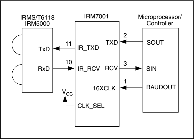
Figure 4. IRM7001 Usage Scenario (with External Clock)
