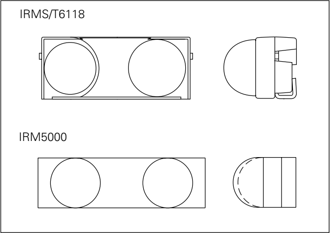
Figure 5. Transceivers IRMS/T6118 and IRM5000
