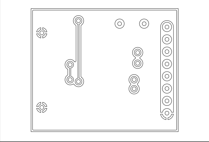
Figure 17. IRMS6118/7001 Eval Board Looking from Back Side
