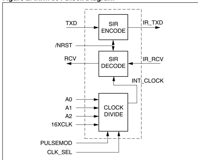
Figure 2. IRM7001 Block Diagram
