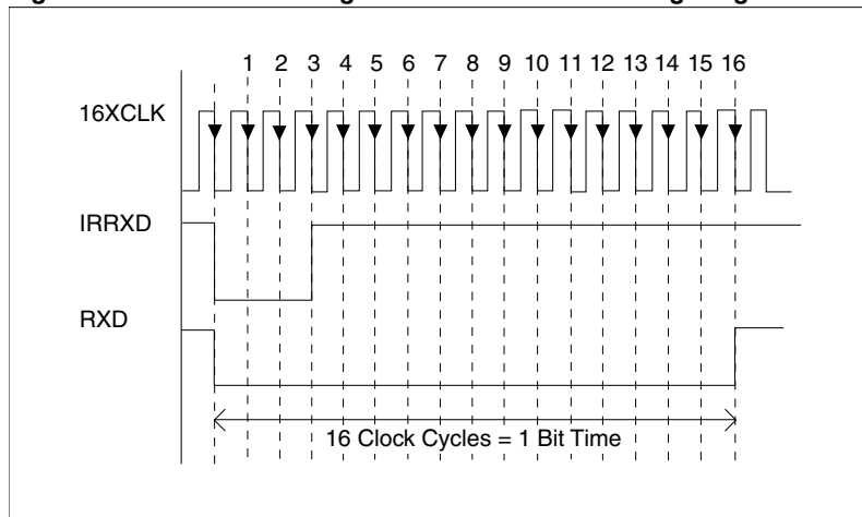
Figure 9. IrDA-SIR Decoding Scheme—Detailed Timing Diagram
