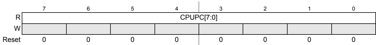
Figure 3-7. Captured S12ZCPU Program Counter (MMCPCH, MMCPCH, MMCPCL)
