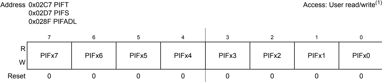
Figure 2-21. Port Interrupt Flag Register
