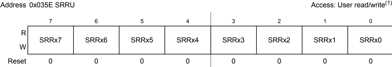
Figure 2-22. Port Slew Rate Register
