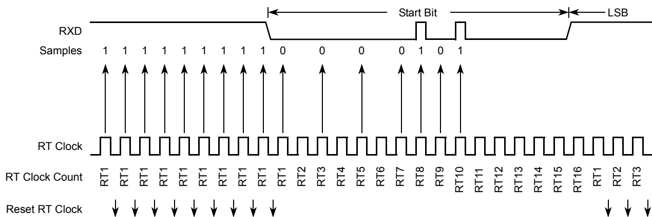
In Figure 12-27 , a noise burst makes the majority of data samples RT8, RT9, and RT10 high. This sets the noise flag but does not reset the RT clock. In start bits only, the RT8, RT9, and RT10 data samples are ignored.
