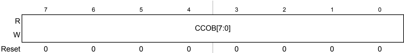
Figure 21-29. Flash Common Command Object 5 Low Register (FCCOB5LO)
