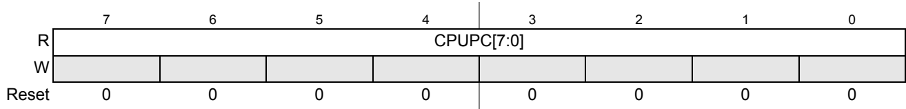
Figure 3-7. Captured S12ZCPU Program Counter (MMCPCH, MMCPCH, MMCPCH)
