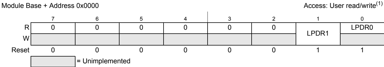
Figure 23-3. Port LP Data Register (LPDR)
