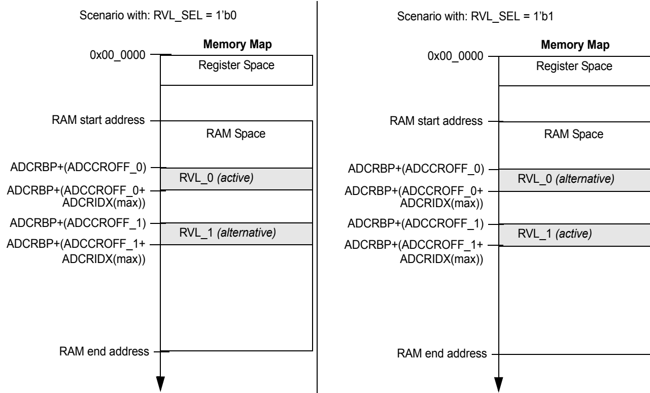
Figure 10-33. Result Value List Schema in Double Buffer Mode
