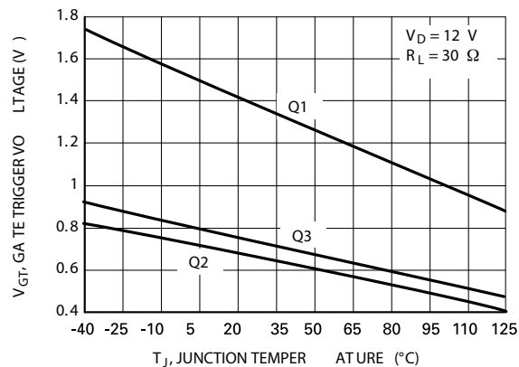
Figure 7. Typical Gate Trigger Voltage Variation
