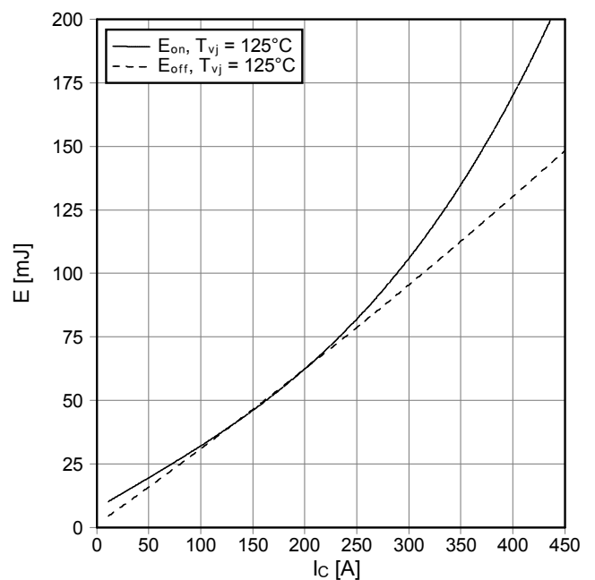
Schaltverluste IGBT-Wechselr. (typisch) switching losses IGBT-inverter (typical) E_{on} = f(I_C) , E_{off} = f(I_C) V_{GE} = \pm 15 \text{ V} , R_{Gon} = 6.2 \Omega , R_{Goff} = 6.2 \Omega , V_{CE} = 900 \text{ V}
