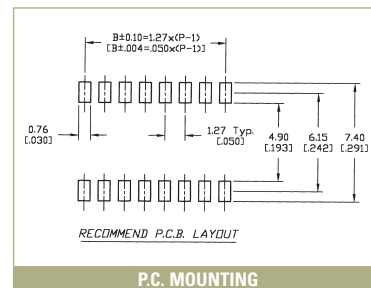
P.C. MOUNTING
