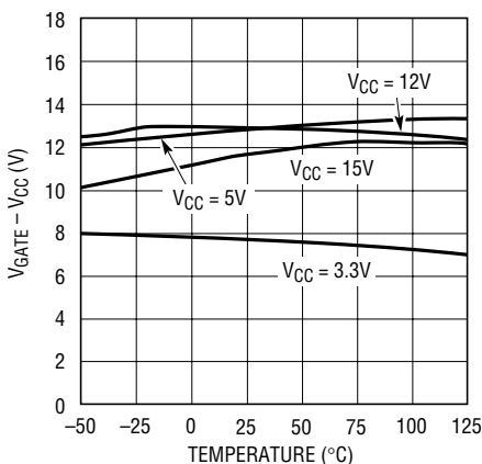
V_{\text{GATE}} - V_{\text{CC}} vs Temperature
