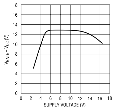
V_{\text{GATE}} - V_{\text{CC}} vs Supply Voltage
