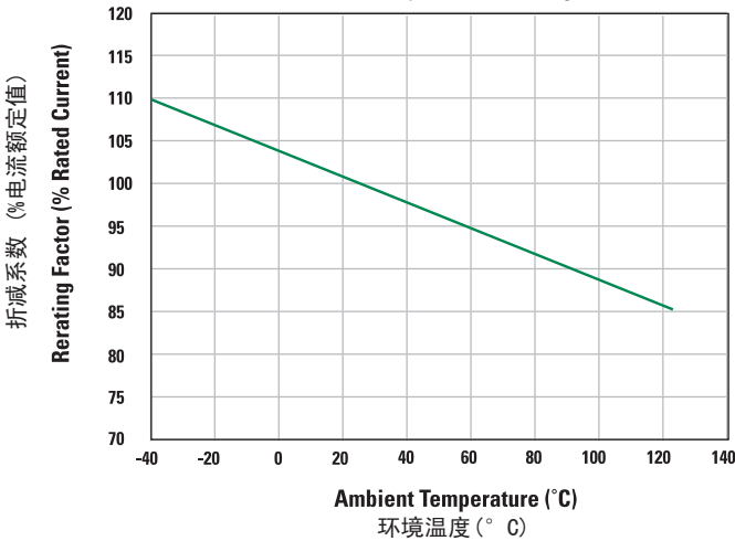
ATOF™ Fuse Temperature Rerating Curve
