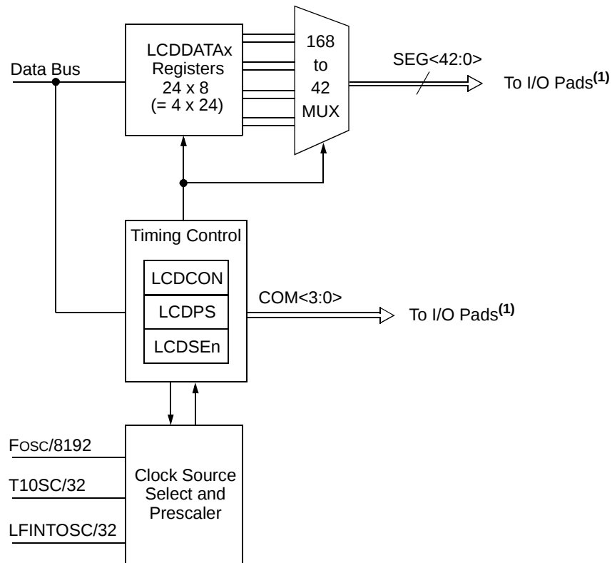
FIGURE 9-1: LCD DRIVER MODULE BLOCK DIAGRAM
