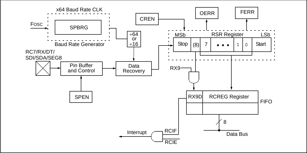
FIGURE 11-5: ASYNCHRONOUS RECEPTION
