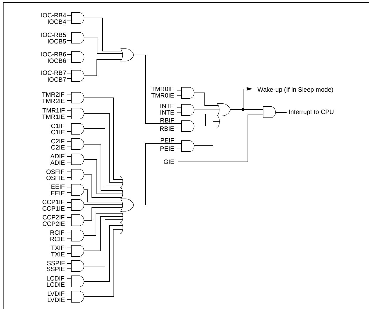
FIGURE 16-7: INTERRUPT LOGIC
