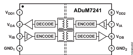
Figure 2. ADuM7241
