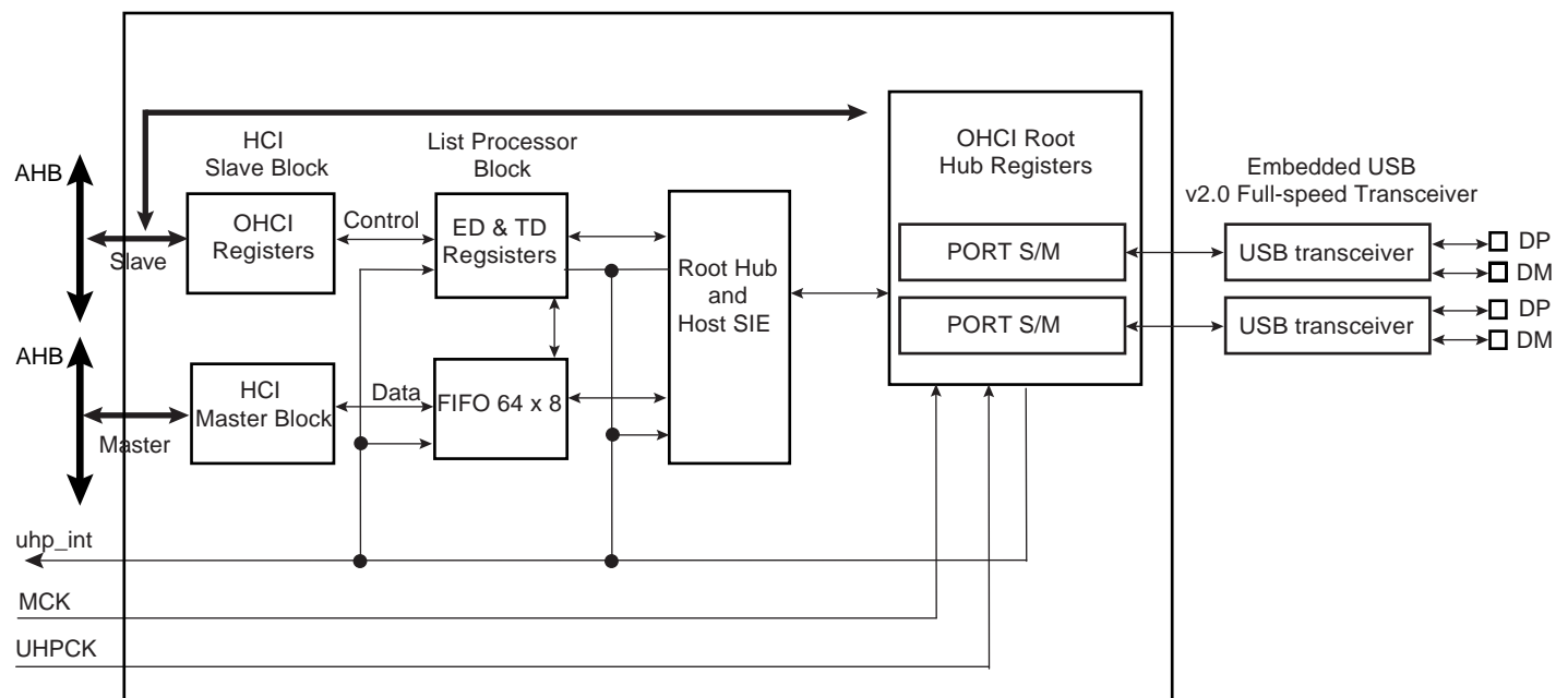
Figure 36-1. Block Diagram
