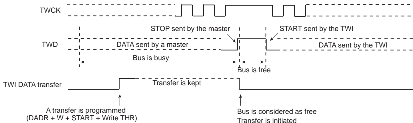
Figure 32-30. User Sends Data While the Bus is Busy
