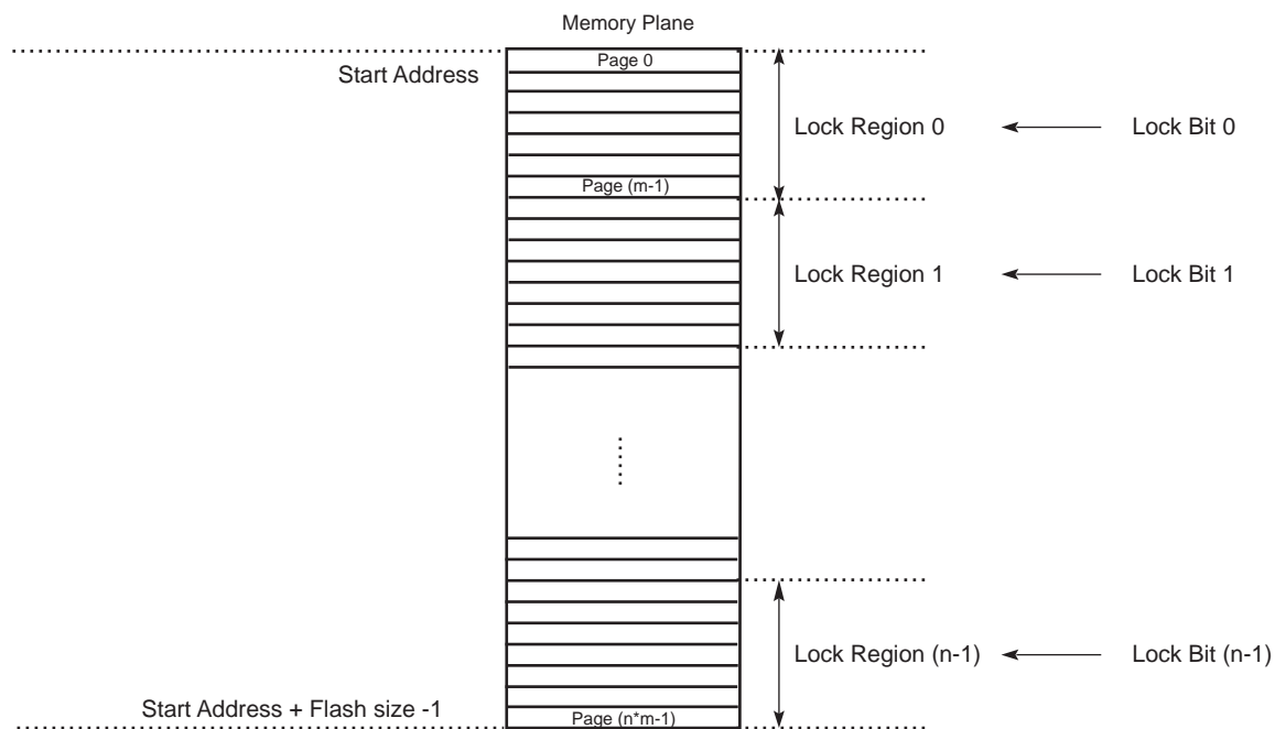
Figure 23-1. Embedded Flash Organization
