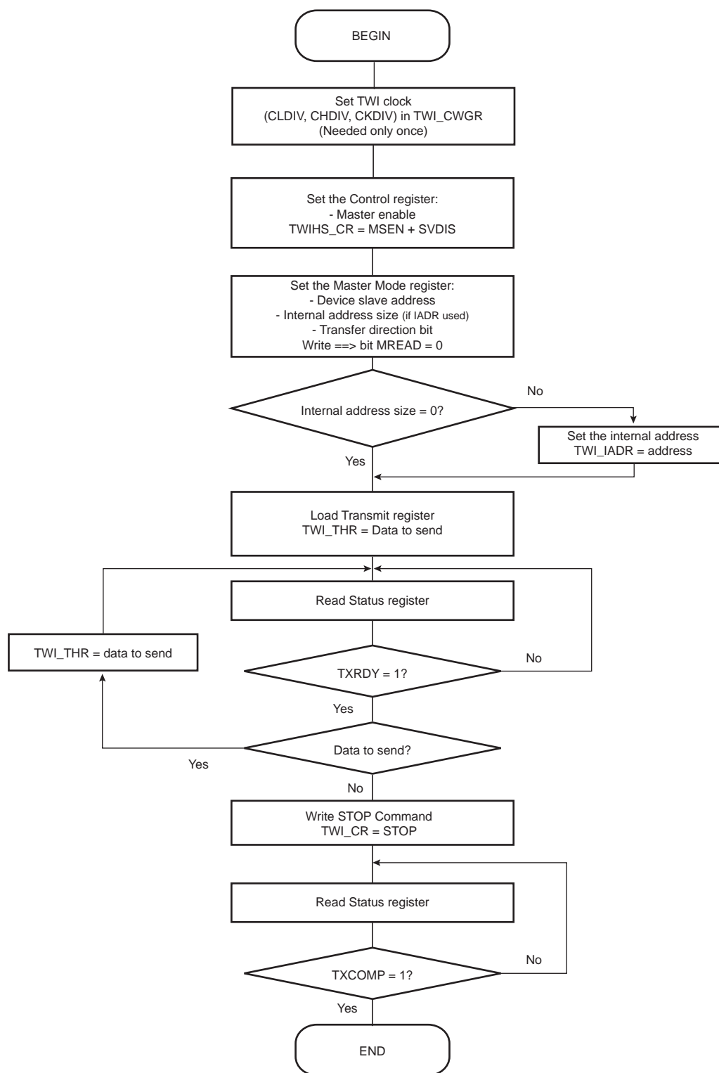
Figure 32-18. TWI Write Operation with Multiple Data Bytes with or without Internal Address
