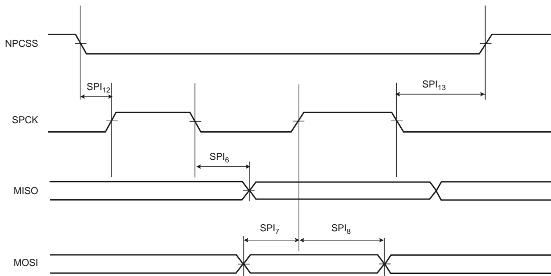
Figure 39-14. SPI Slave Mode with (CPOL = 0 and NCPHA = 1) or (CPOL = 1 and NCPHA = 0)
