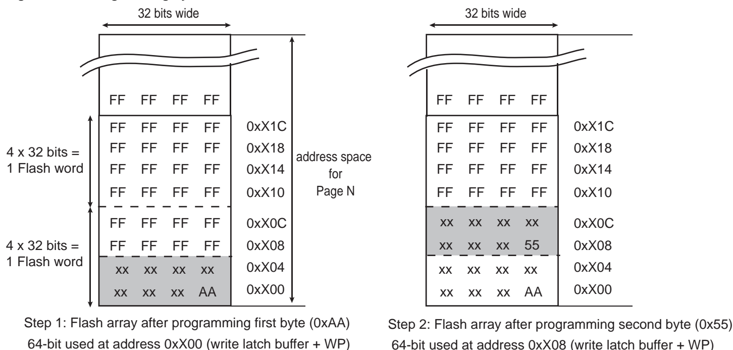
Figure 23-10. Programming Bytes in the Flash
