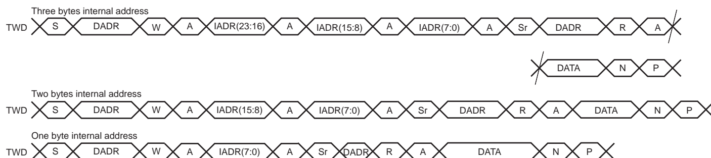
Figure 32-13. Master Read with One, Two or Three Bytes Internal Address and One Data Byte
