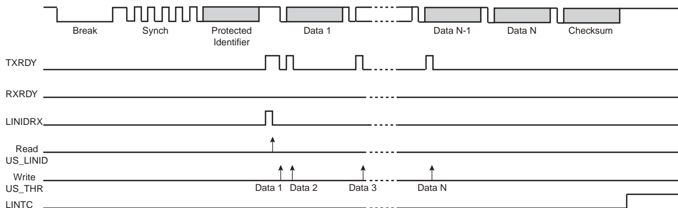
Figure 30-41. Slave Node Configuration, NACT = PUBLISH
