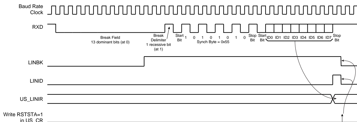
Figure 30-33. Header Reception
