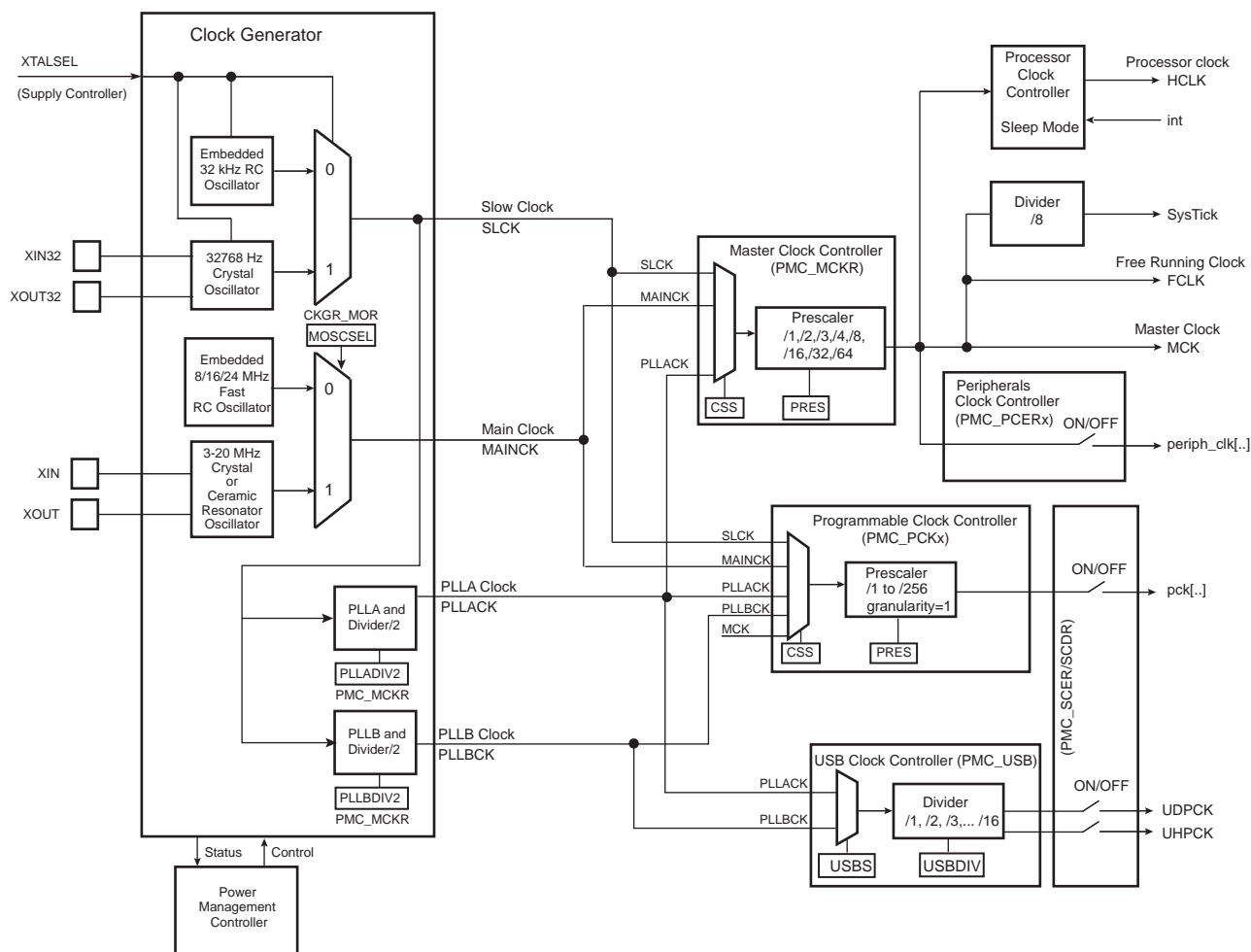
Figure 18-1. General Clock Block Diagram
