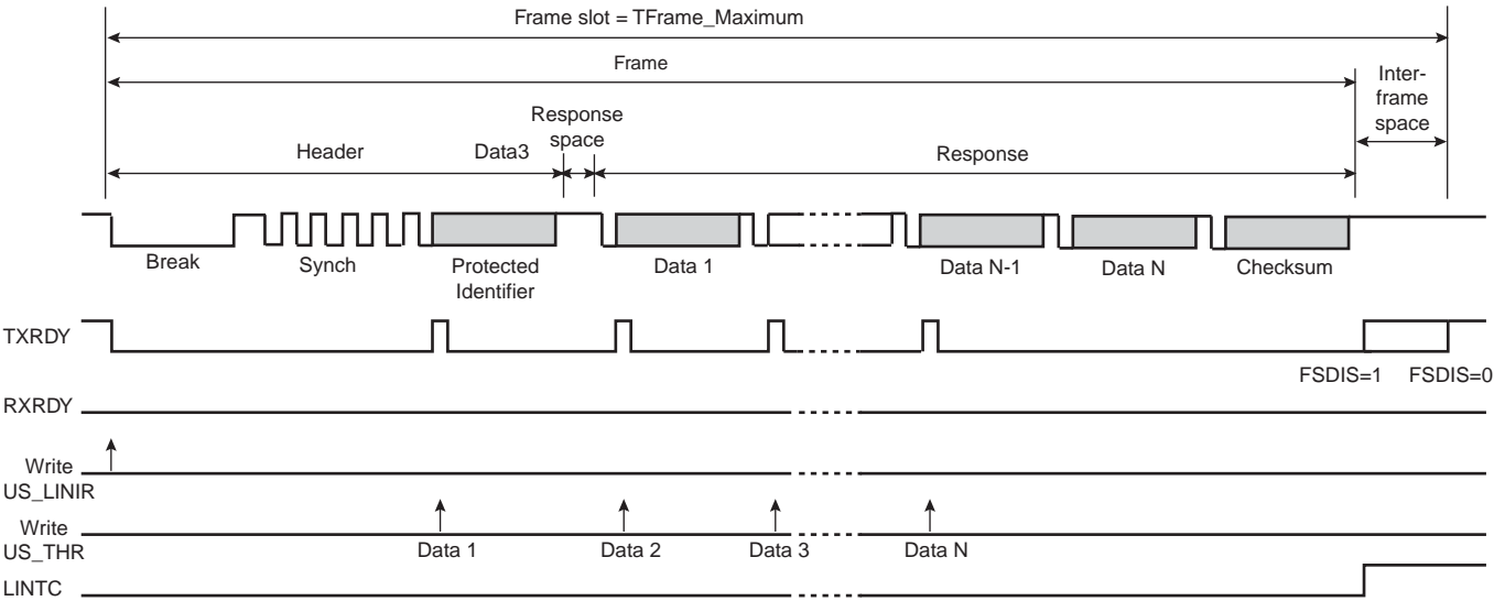
Figure 30-38. Master Node Configuration, NACT = PUBLISH
