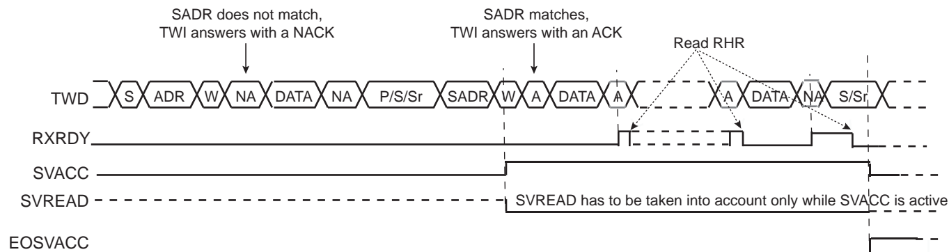
Figure 32-36. Write Access Ordered by a Master
