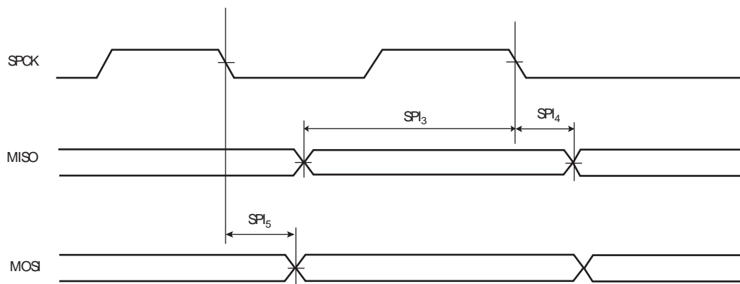
Figure 39-13. SPI Master Mode with (CPOL = 0 and NCPHA=1) or (CPOL=1 and NCPHA= 0)
