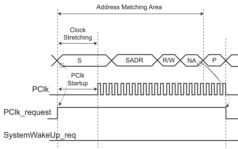
Figure 32-44. No Address Match (Data Matching Disabled)
