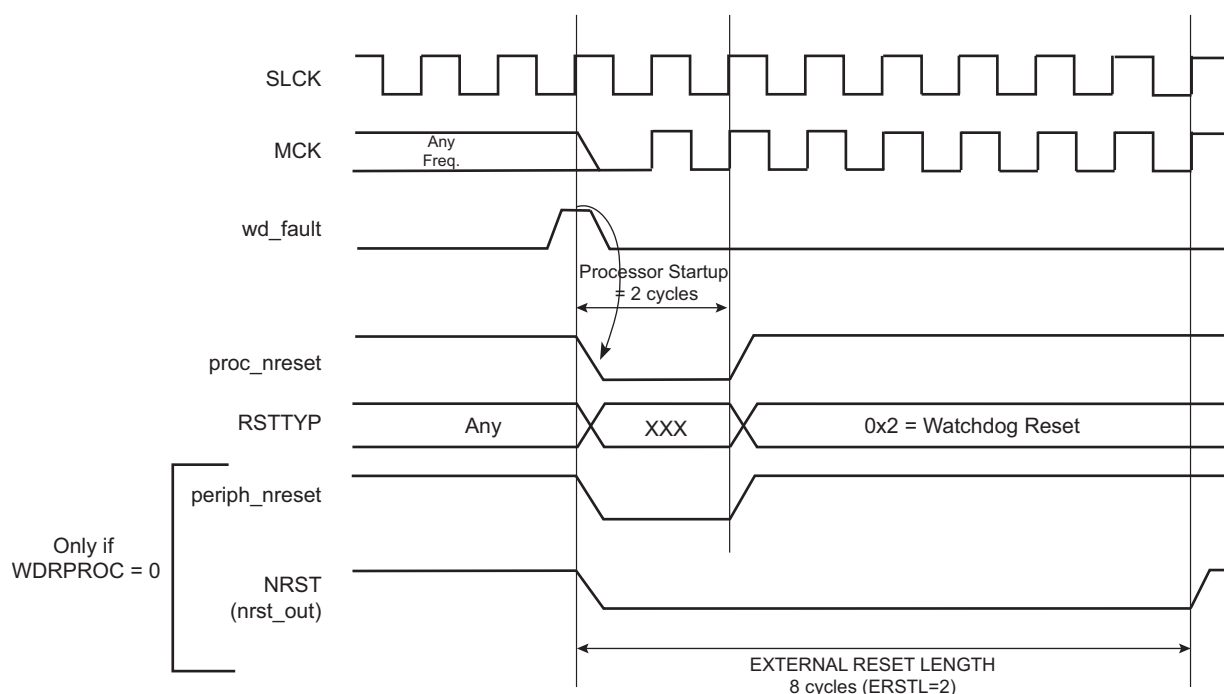
Figure 19-5. Watchdog Reset
