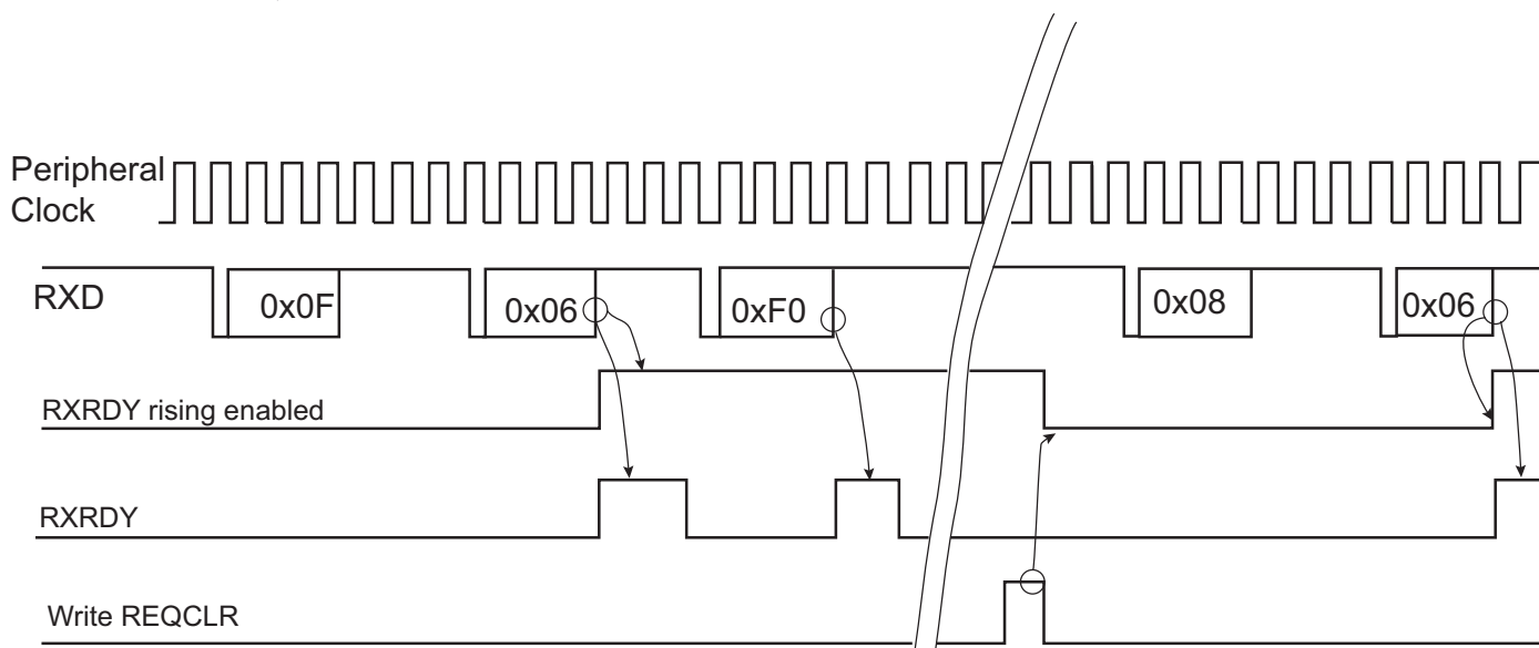
Figure 30-27. Receive Holding Register Management
