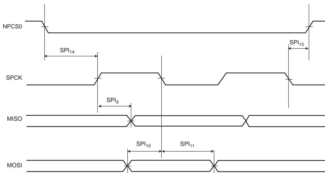
Figure 39-18. USART SPI Slave Mode (Mode 0 or 3)
