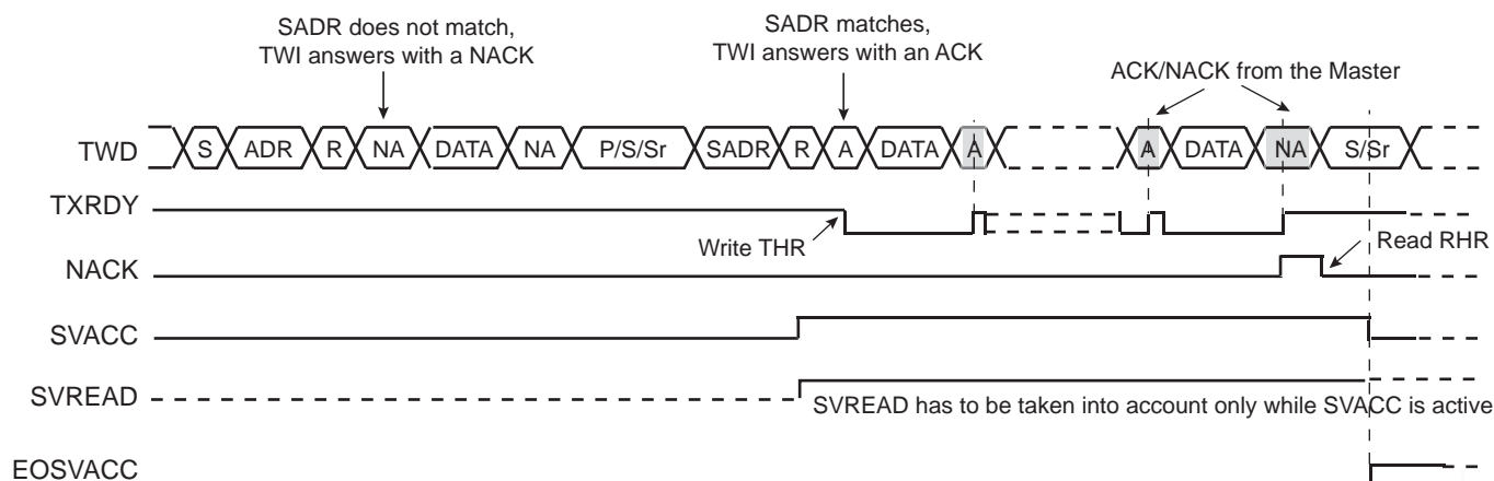
Figure 32-35. Read Access Ordered by a Master
