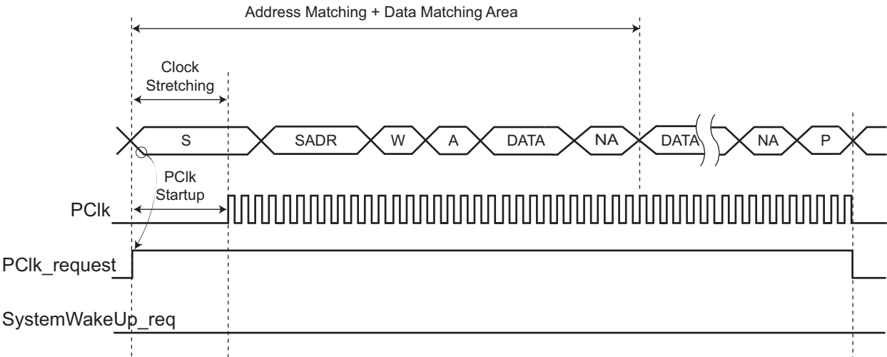
Figure 32-46. Address Match and No Data Match (Data Matching Enabled)
