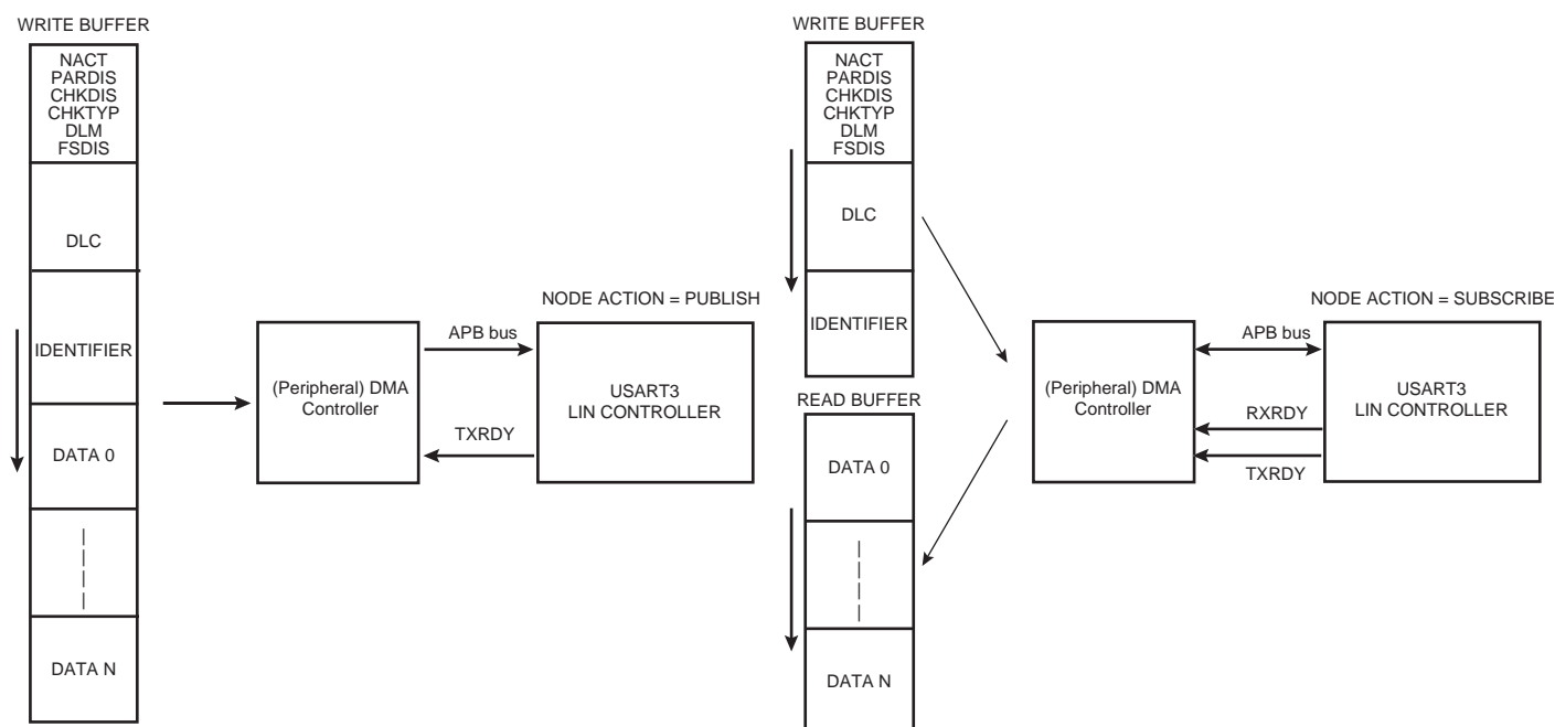
Figure 30-44. Master Node with PDC (PDCM = 1)
