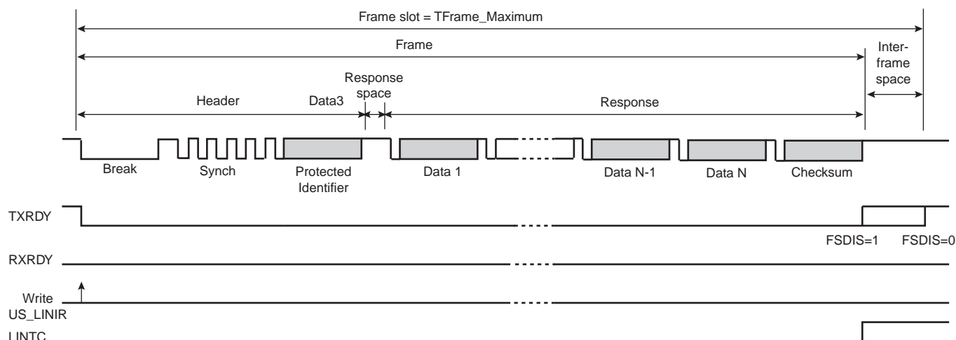
Figure 30-40. Master Node Configuration, NACT = IGNORE
