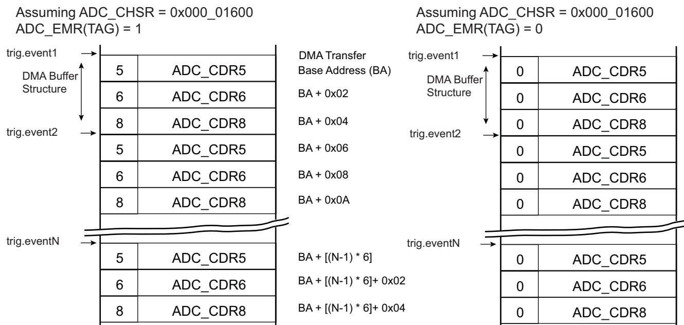
Figure 38-13. Buffer Structure
