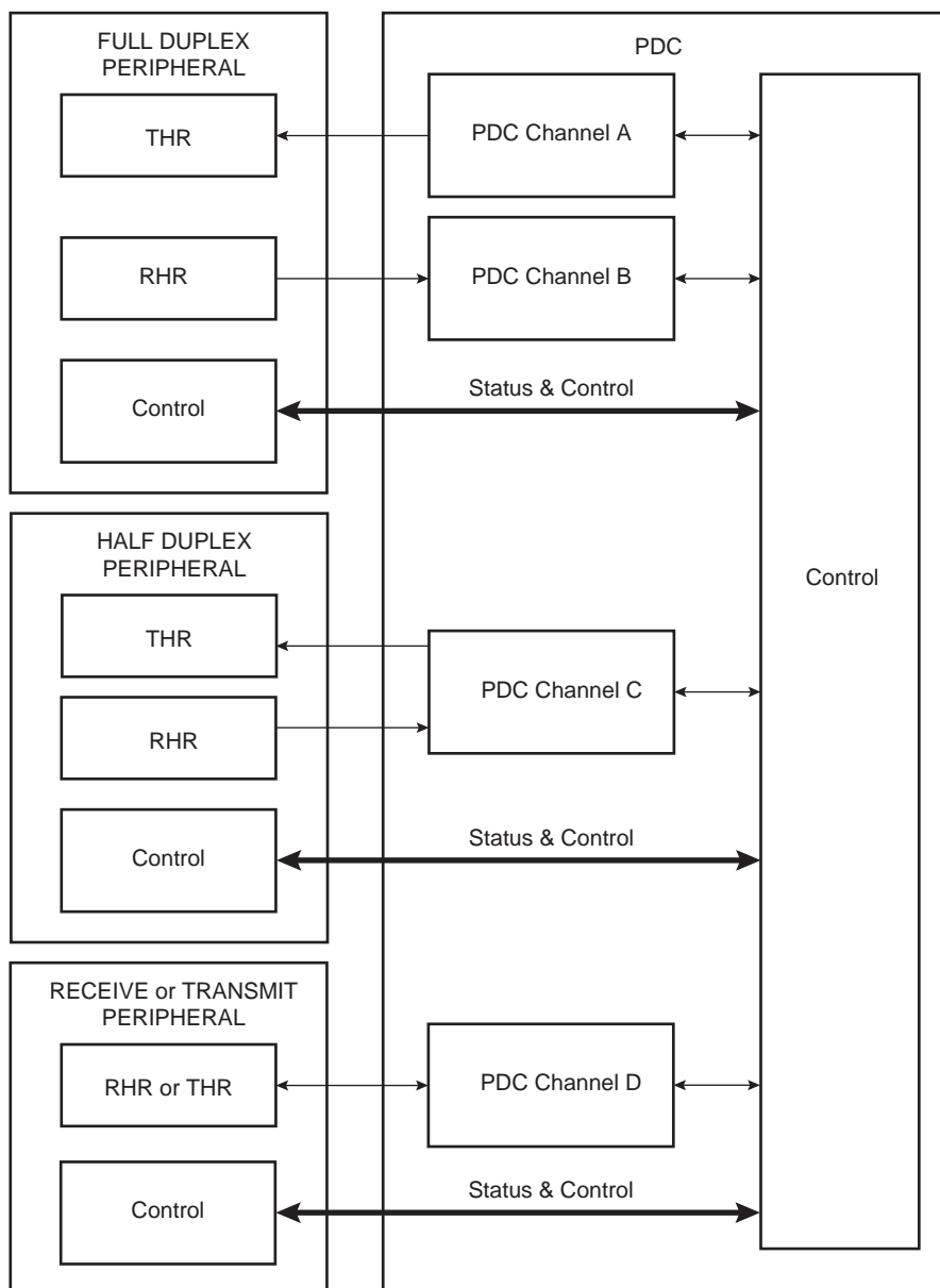
Figure 21-1. Block Diagram
