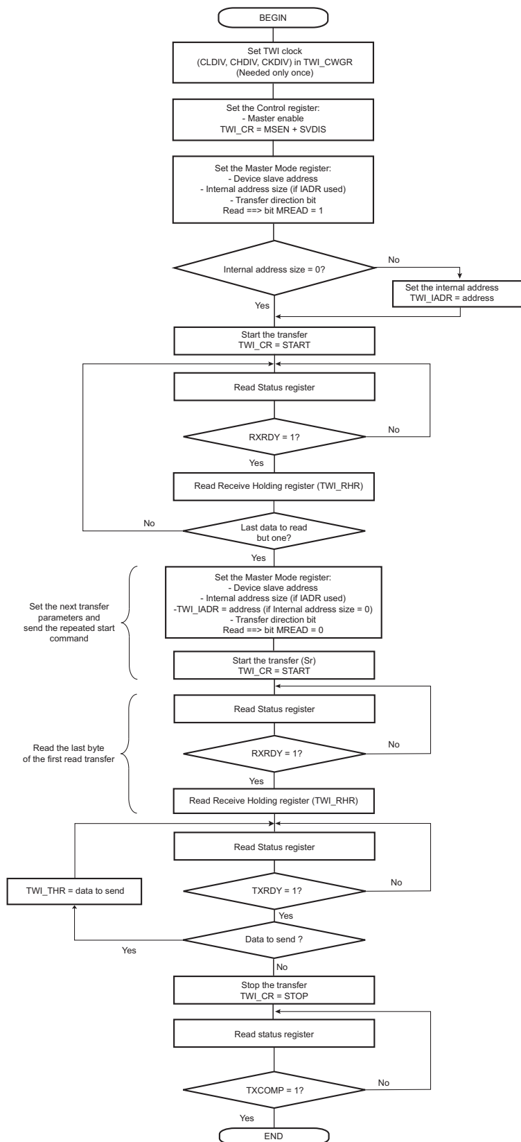
Figure 32-28. TWI Read Operation with Multiple Data Bytes + Write Operation with Multiple Data Bytes (Sr)
