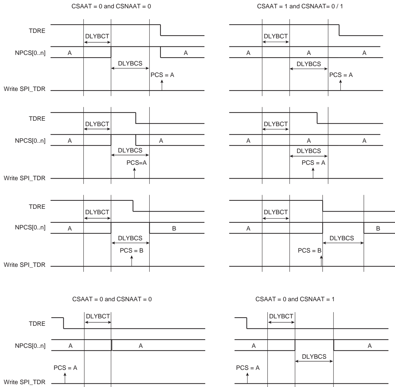
Figure 31-12. Peripheral Deselection
