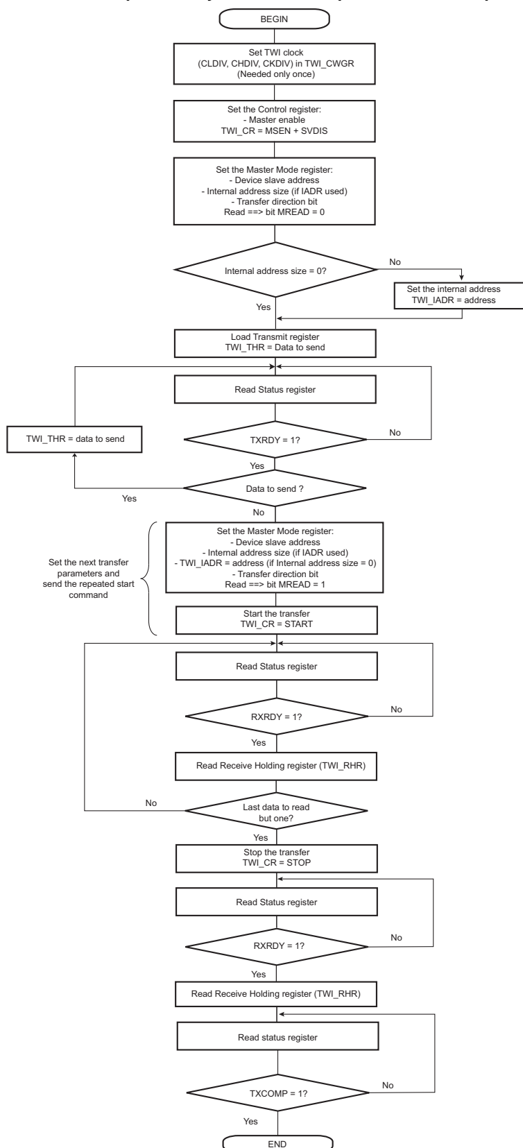
Figure 32-21. TWI Write Operation with Multiple Data Bytes and Read Operation with Multiple Data Bytes (Sr)
