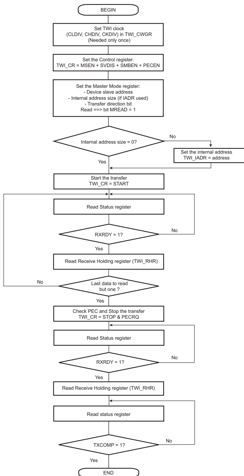
Figure 32-26. TWI Read Operation with Multiple Data Bytes with or without Internal Address with PEC
