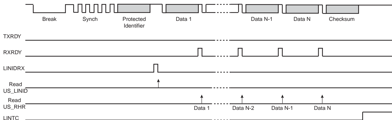
Figure 30-42. Slave Node Configuration, NACT = SUBSCRIBE
