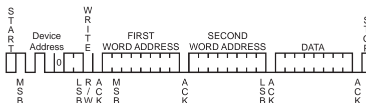
Figure 32-14. Internal Address Usage
