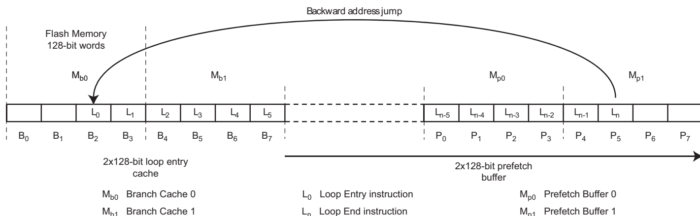
Figure 23-4. Code Loop Optimization
