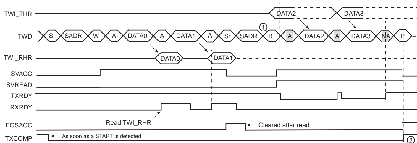
Figure 32-41. Repeated Start and Reversal from Write Mode to Read Mode
