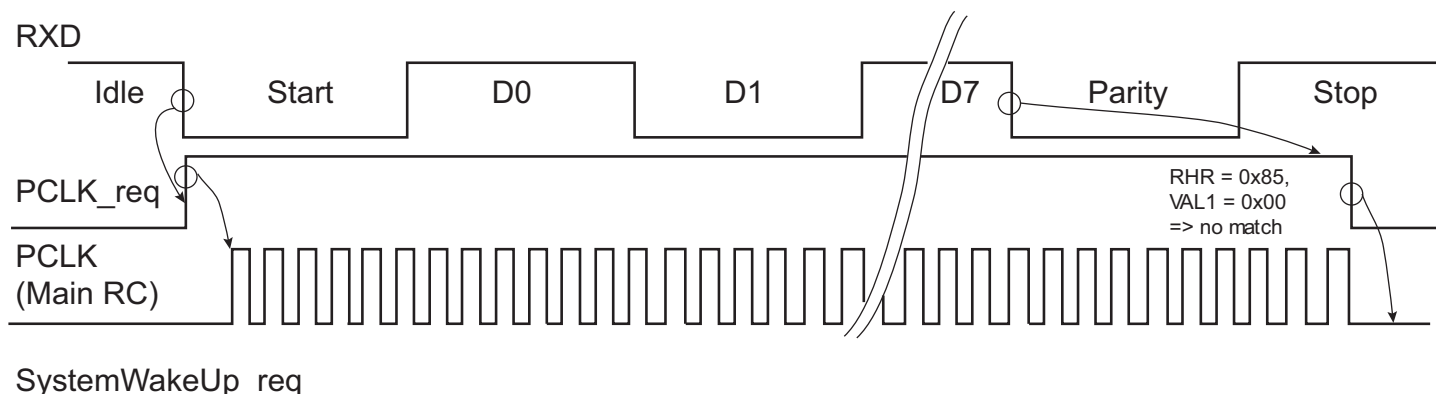
Figure 30-29. Asynchronous Event Generating Only Partial Wake-up Case with VAL1 = VAL2 = 0x00, CMPPAR = Don't care
