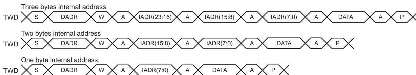
Figure 32-12. Master Write with One, Two or Three Bytes Internal Address and One Data Byte
