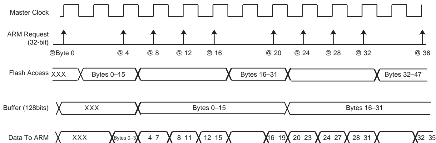
Figure 23-5. Data Read Optimization for FWS = 1
