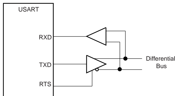
Figure 30-25. Typical Connection to a RS485 Bus
