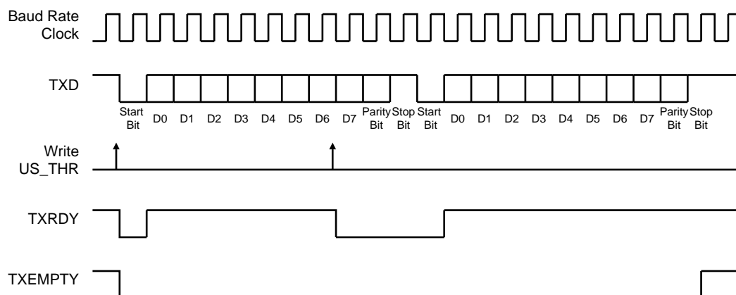
Figure 30-6. Transmitter Status
