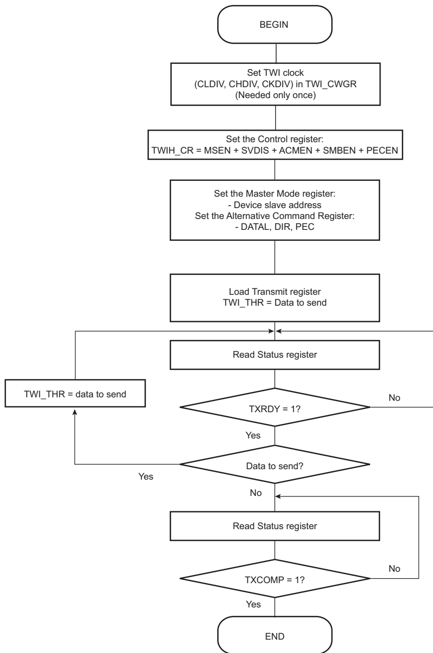
Figure 32-20. SMBus Write Operation with Multiple Data Bytes with PEC and Alternative Command Mode
