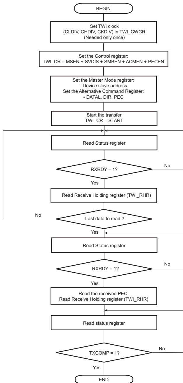
Figure 32-27. TWI Read Operation with Multiple Data Bytes with Alternative Command Mode with PEC
