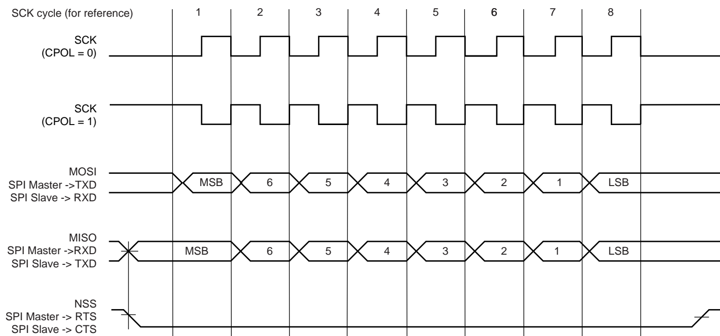
Figure 30-30. SPI Transfer Format (CPHA = 1, 8 bits per transfer)
