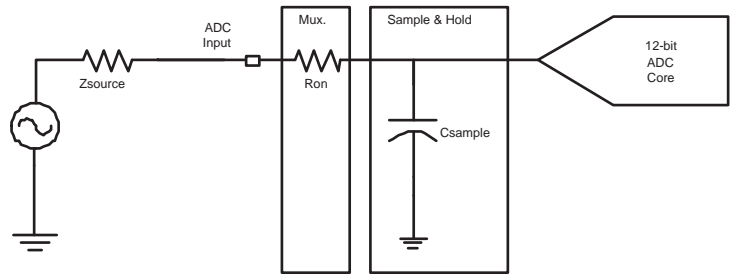
Figure 39-10. Simplified Acquisition Path
