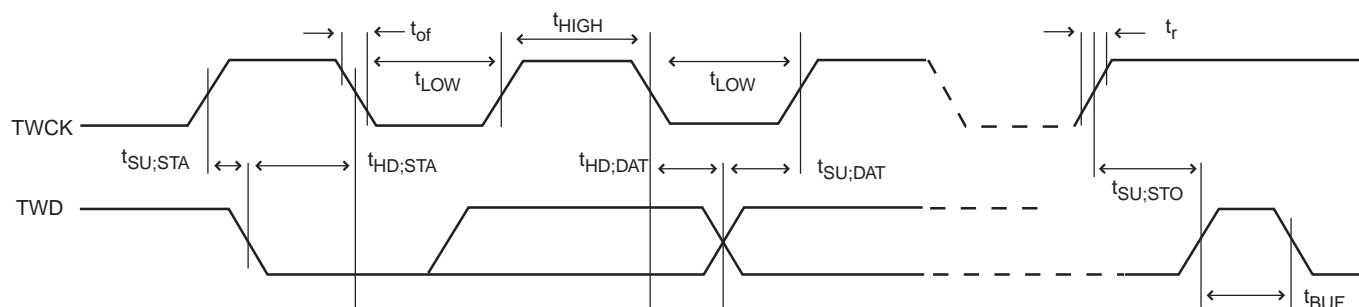
Figure 39-19. Two-wire Serial Bus Timing
