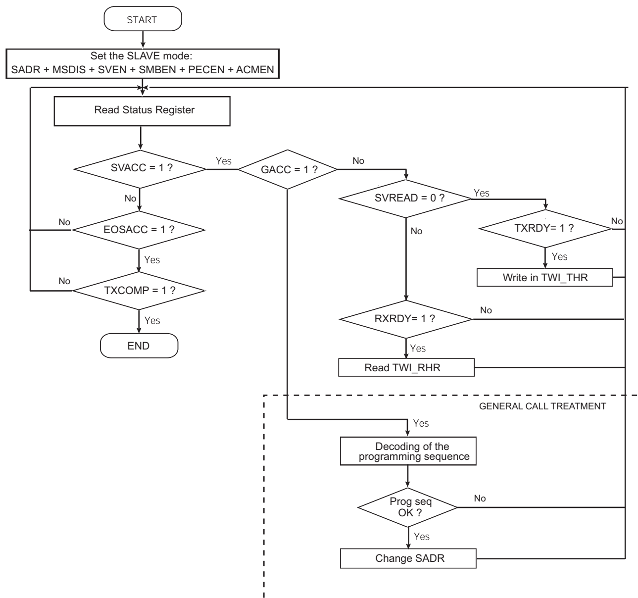
Figure 32-49. Read Write Flowchart in Slave Mode with SMBus PEC and Alternative Command Mode
