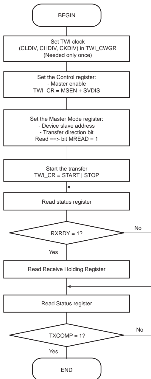
Figure 32-23. TWI Read Operation with Single Data Byte without Internal Address
