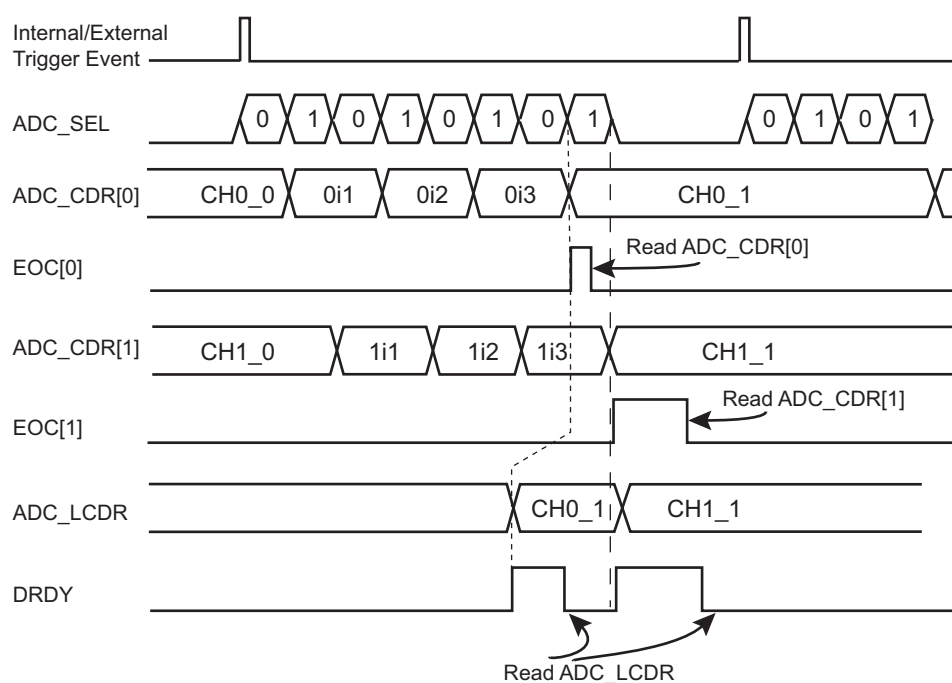
Figure 38-11. Digital Averaging Function Waveforms on a Single Trigger Event
