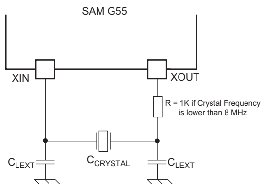
Figure 39-9. 3 to 20 MHz Crystal Oscillator Schematic
