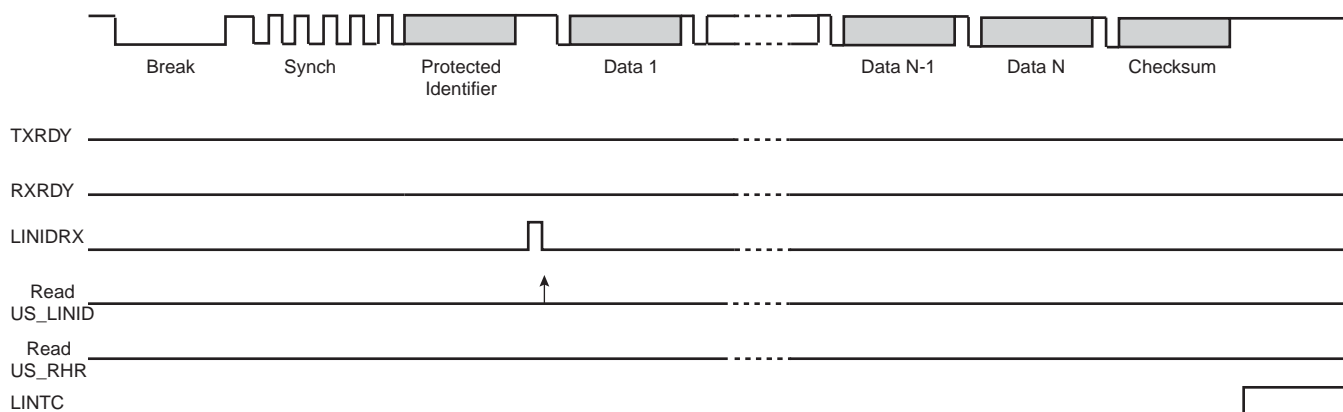
Figure 30-43. Slave Node Configuration, NACT = IGNORE
