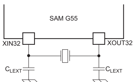
Figure 39-8. 32.268 kHz Crystal Oscillator Schematic
