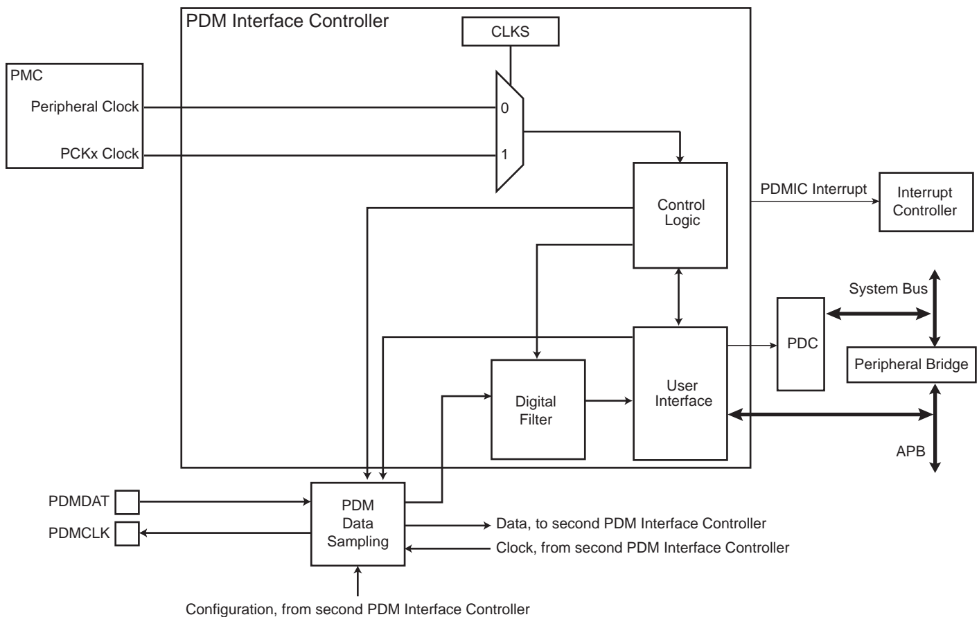
Figure 34-1. Pulse Density Modulation Interface Controller Block Diagram
