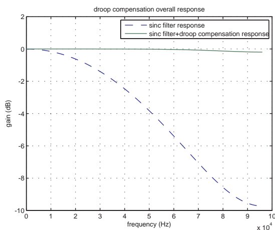
Figure 34-5. Droop Compensation Filter Overall Frequency Response
