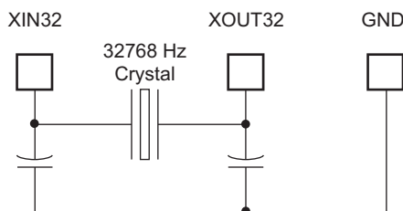
Figure 17-2. Typical Slow Clock Crystal Oscillator Connection
