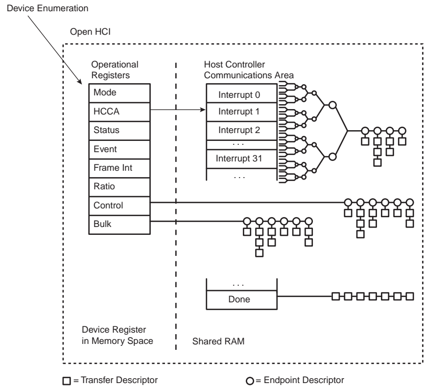
Figure 36-2. USB Host Communication Channels
