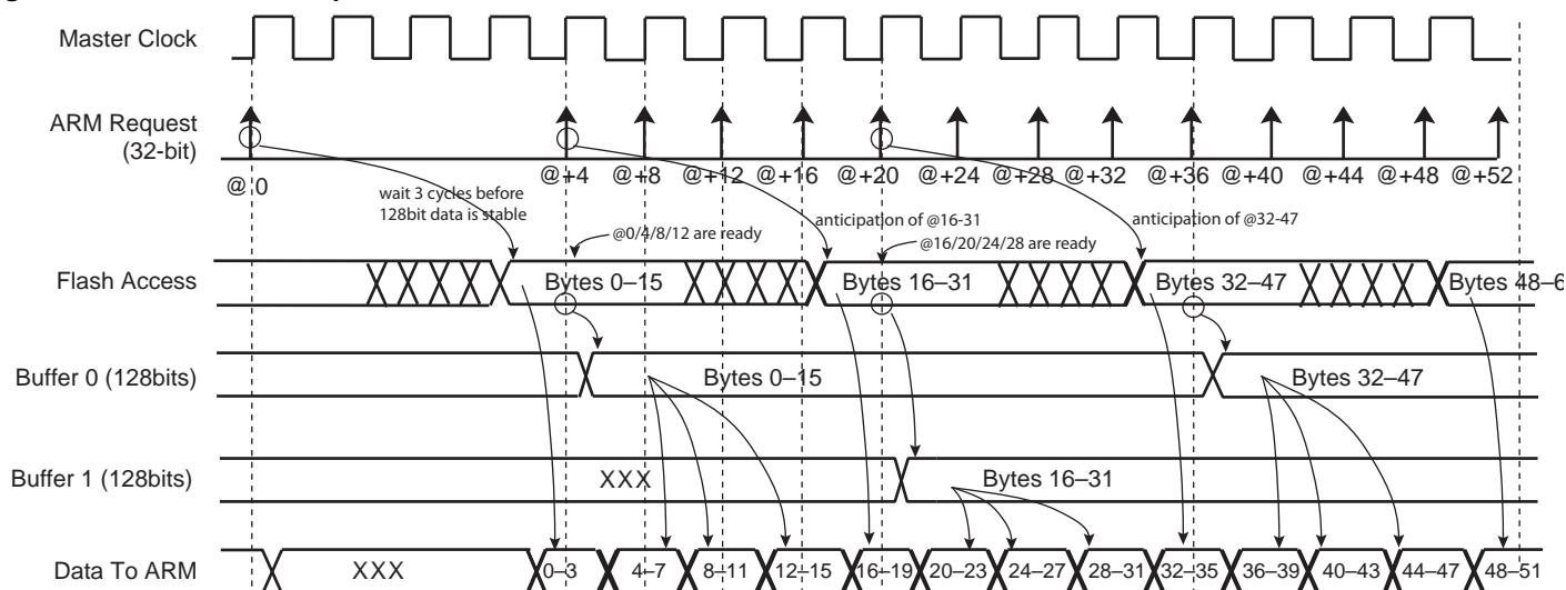
Figure 23-3. Code Read Optimization for FWS = 3
