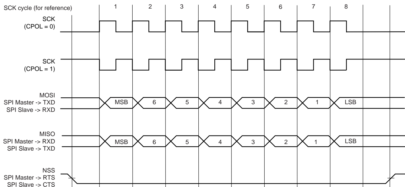
Figure 30-31. SPI Transfer Format (CPHA = 0, 8 bits per transfer)
