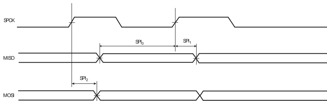
Figure 39-12. SPI Master Mode with (CPOL= NCPHA = 0) or (CPOL= NCPHA= 1)
