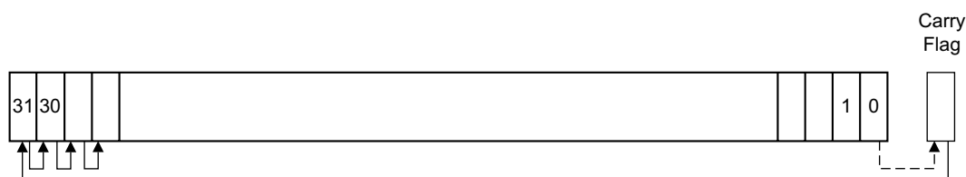
Figure 13-12. RRX
