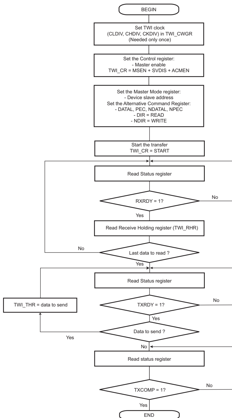
Figure 32-29. TWI Read Operation with Multiple Data Bytes + Write with Alternative Command Mode with PEC
