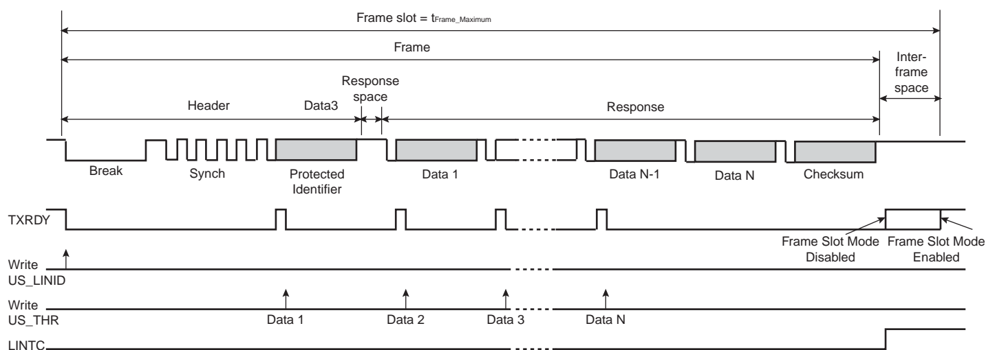
Figure 30-37. Frame Slot Mode
