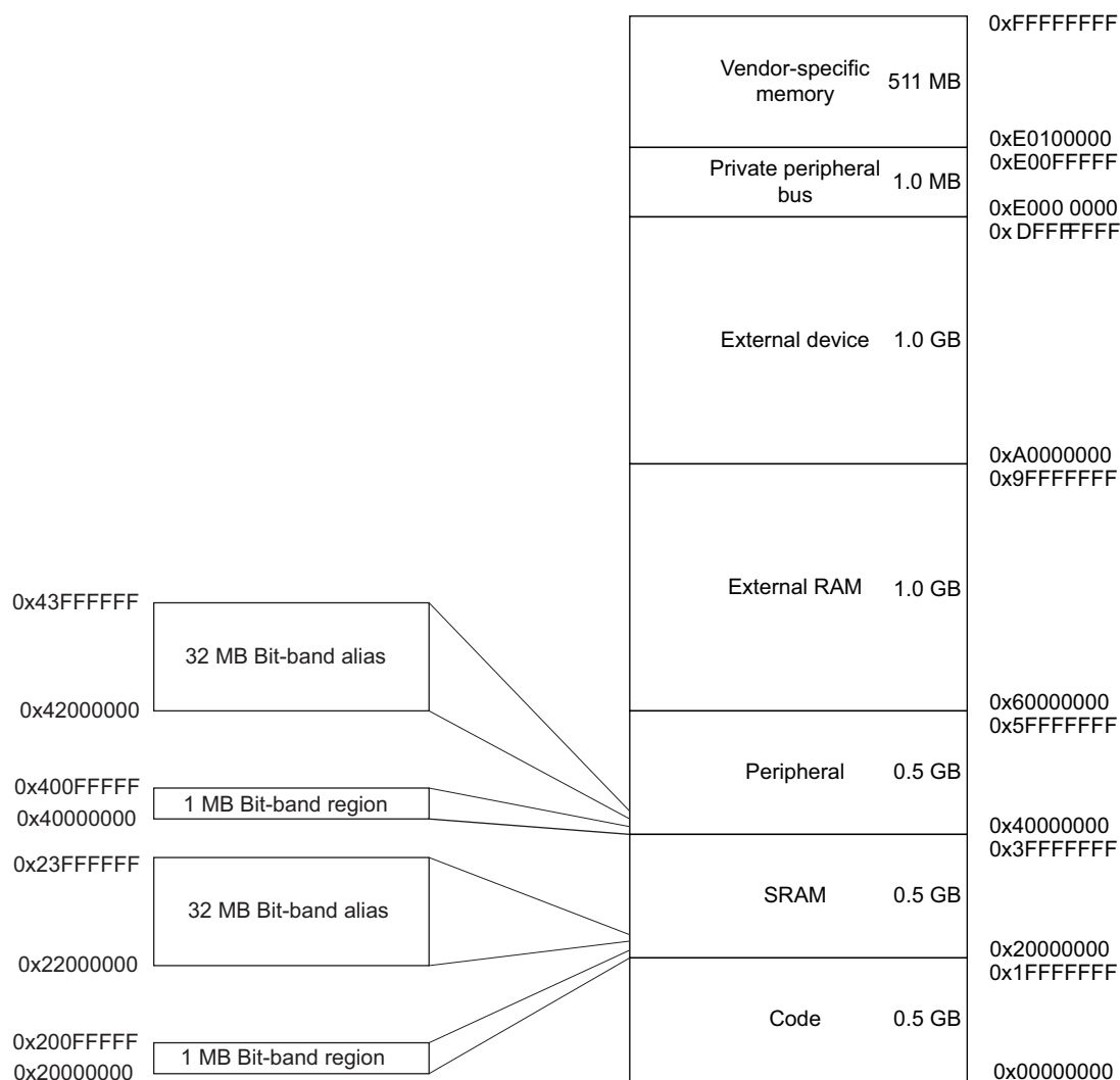
Figure 13-3. Memory Map
