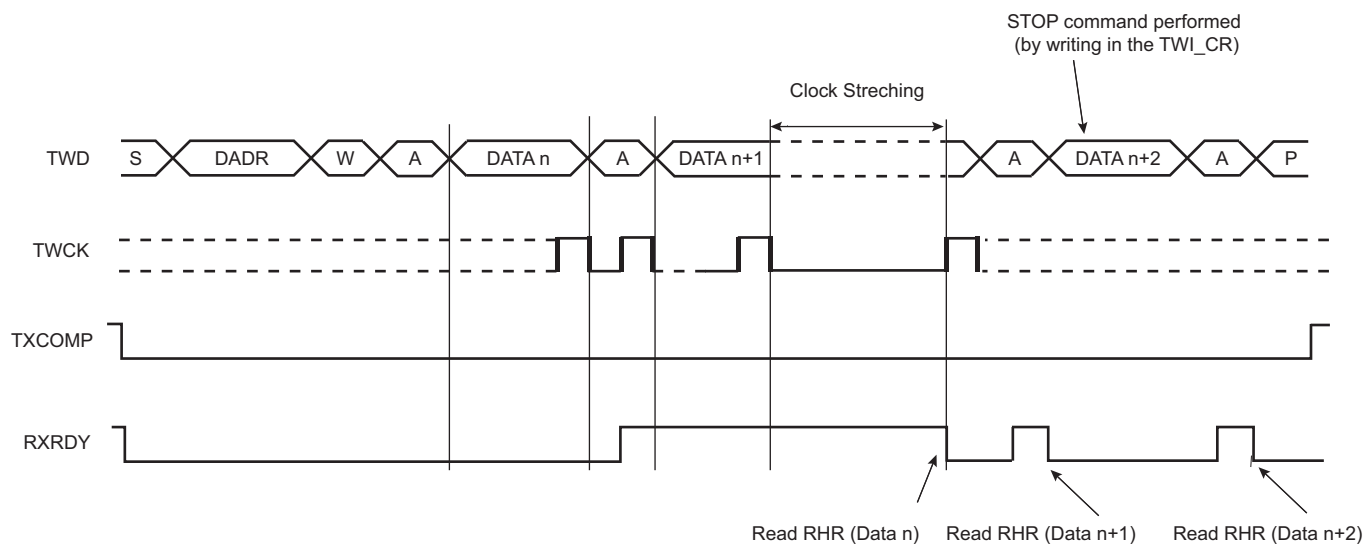
Figure 32-11. Master Read Clock Stretching with Multiple Data Bytes
