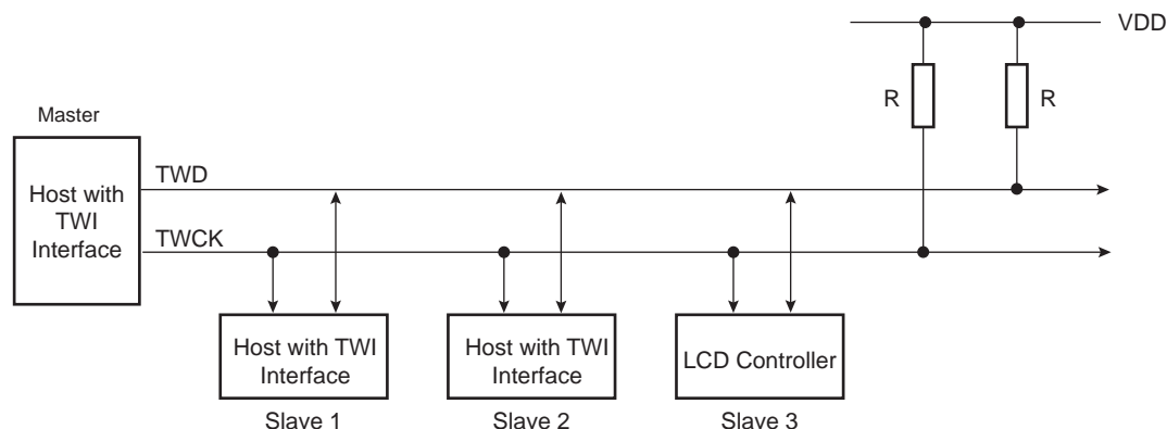
Figure 32-34. Fast Mode Slave Mode Typical Application Block Diagram
