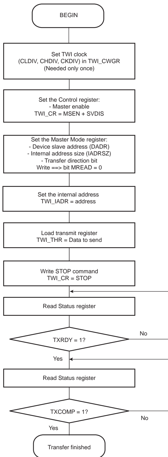
Figure 32-17. TWI Write Operation with Single Data Byte and Internal Address
