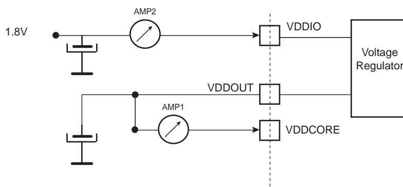
Figure 39-7. Active Mode Measurement Setup
