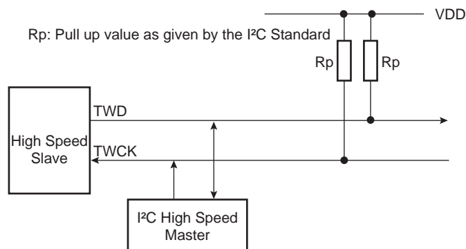
Figure 32-33. High-Speed Mode Slave Mode Typical Application Block Diagram
