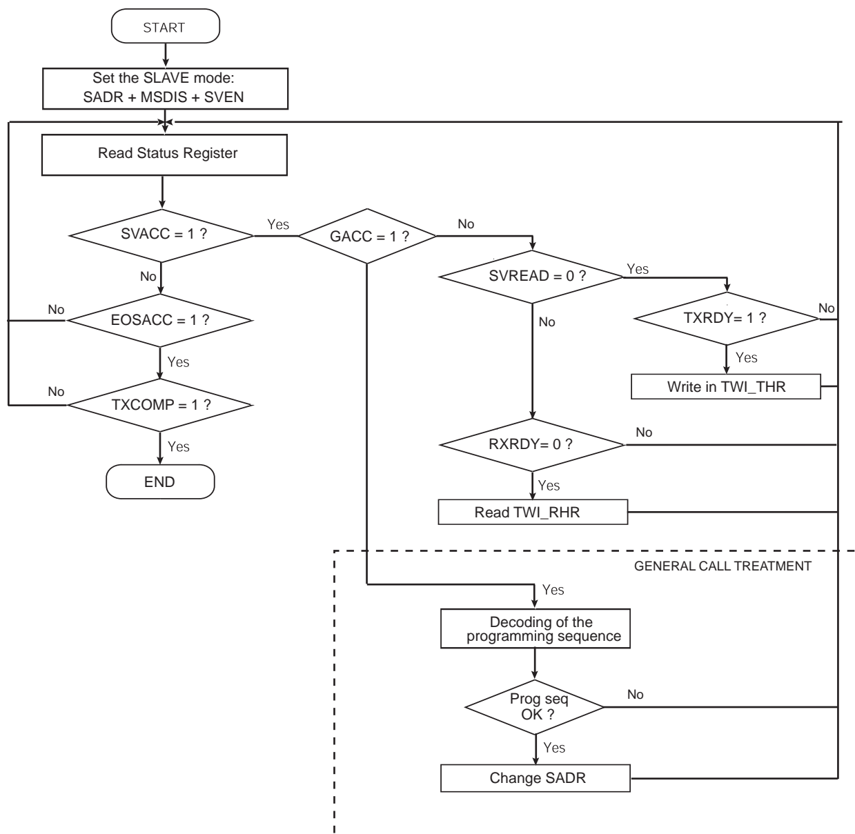
Figure 32-47. Read Write Flowchart in Slave Mode
