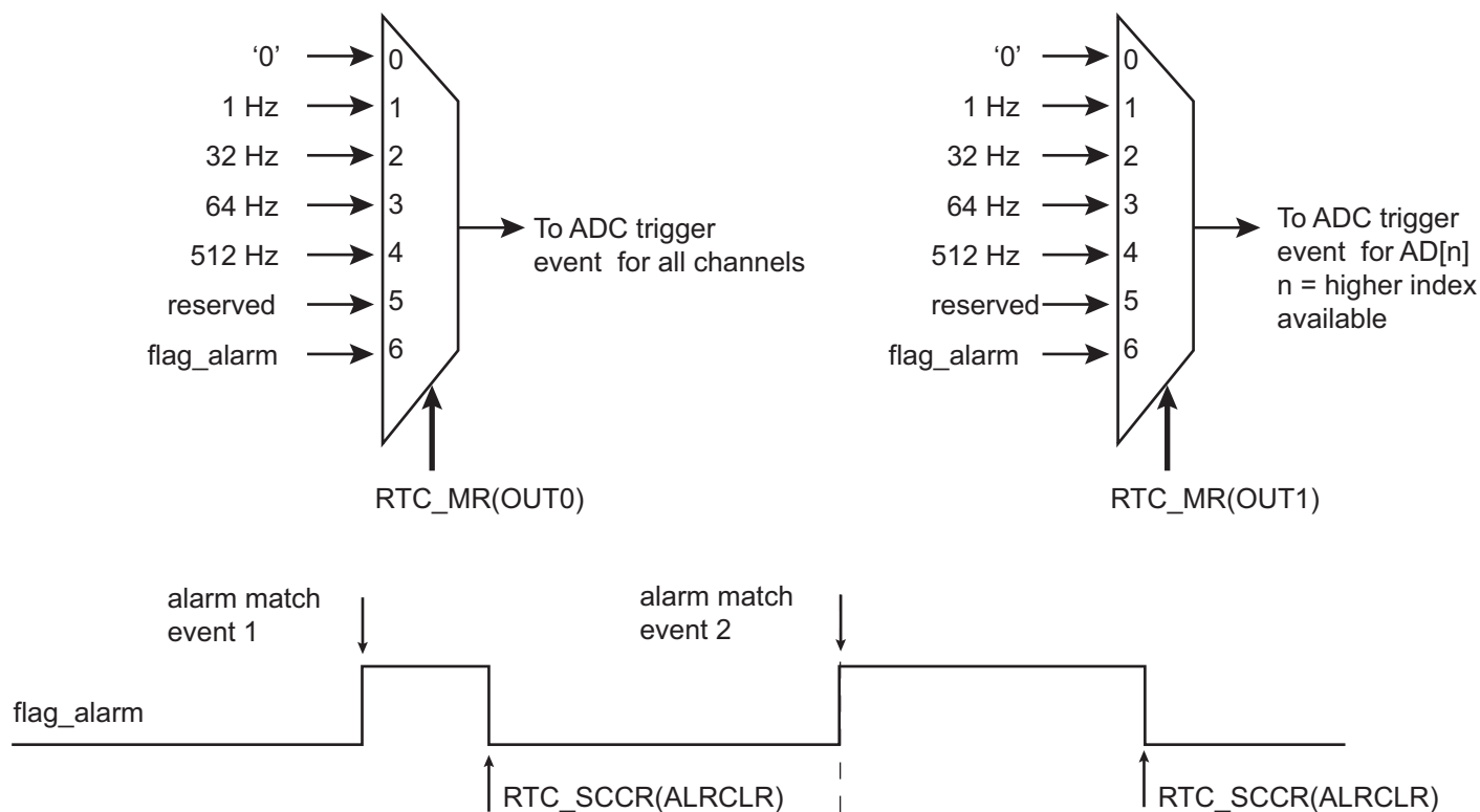
Figure 26-3. Waveform Generation for ADC Trigger Event
