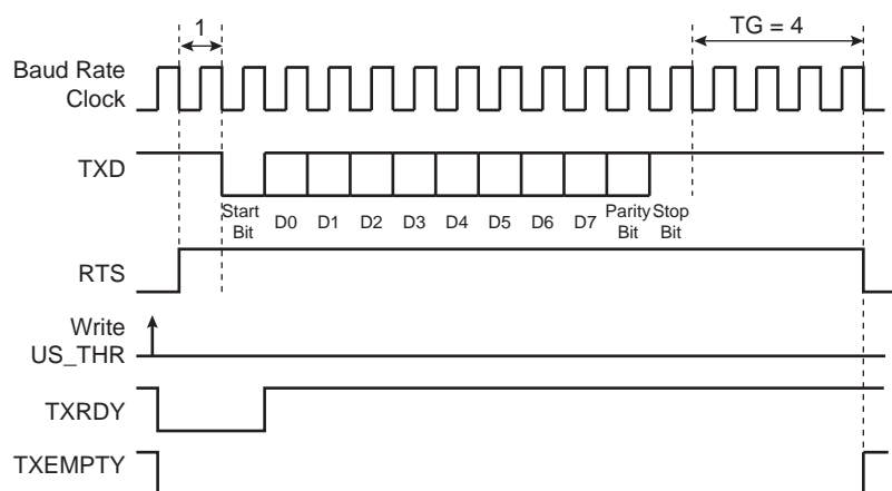
Figure 30-26. Example of RTS Drive with Timeguard
