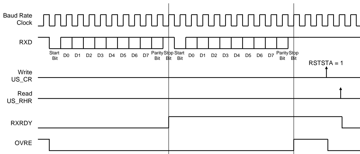
Figure 30-10. Receiver Status
