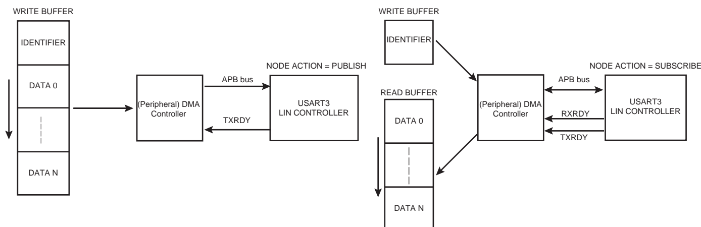
Figure 30-45. Master Node with PDC (PDCM = 0)
