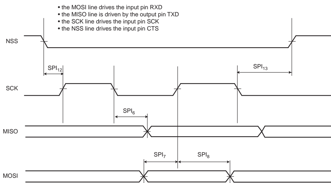
Figure 39-17. USART SPI Slave Mode (Mode 1 or 2)
