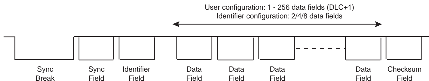
Figure 30-36. Response Data Length
