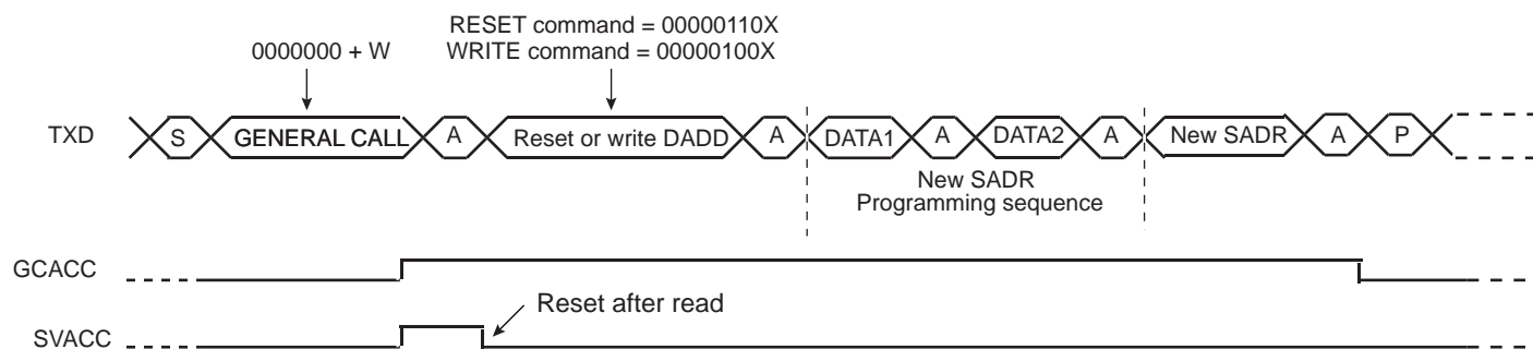
Figure 32-37. Master Performs a General Call
