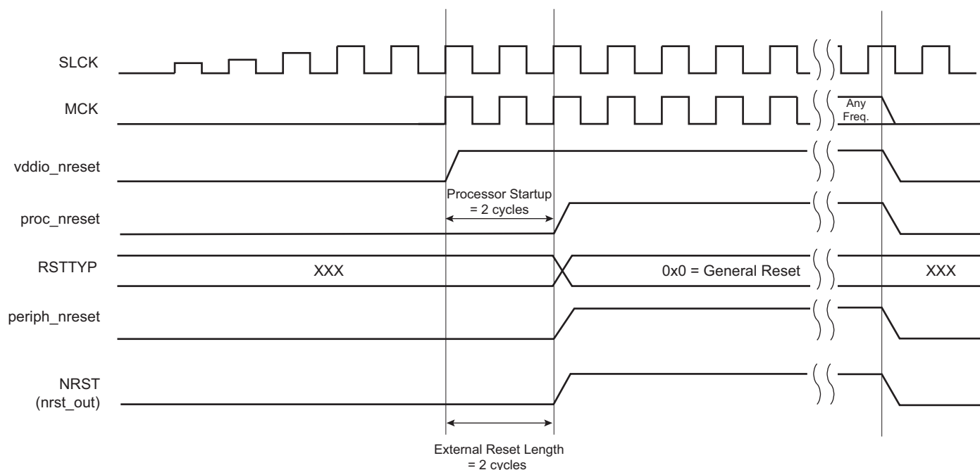
Figure 19-3. General Reset State
