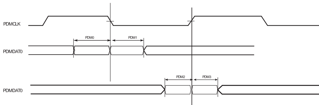
Figure 39-11. PDM Mode
