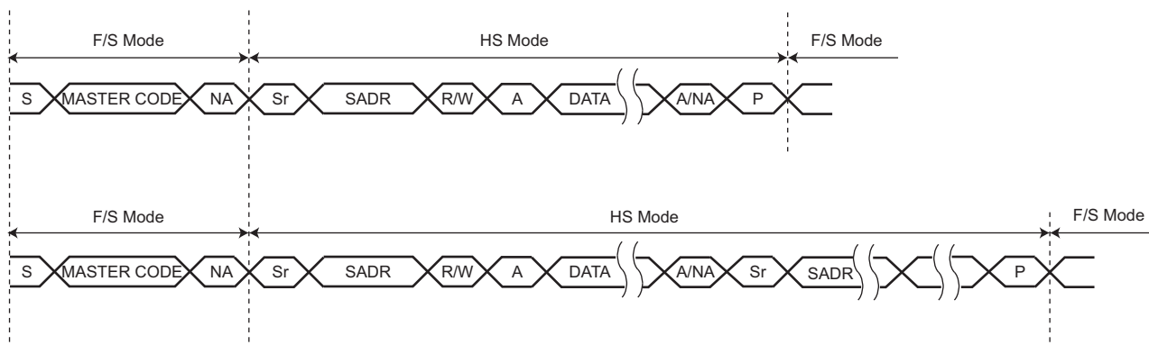
Figure 32-42. High-Speed Mode Read/Write
