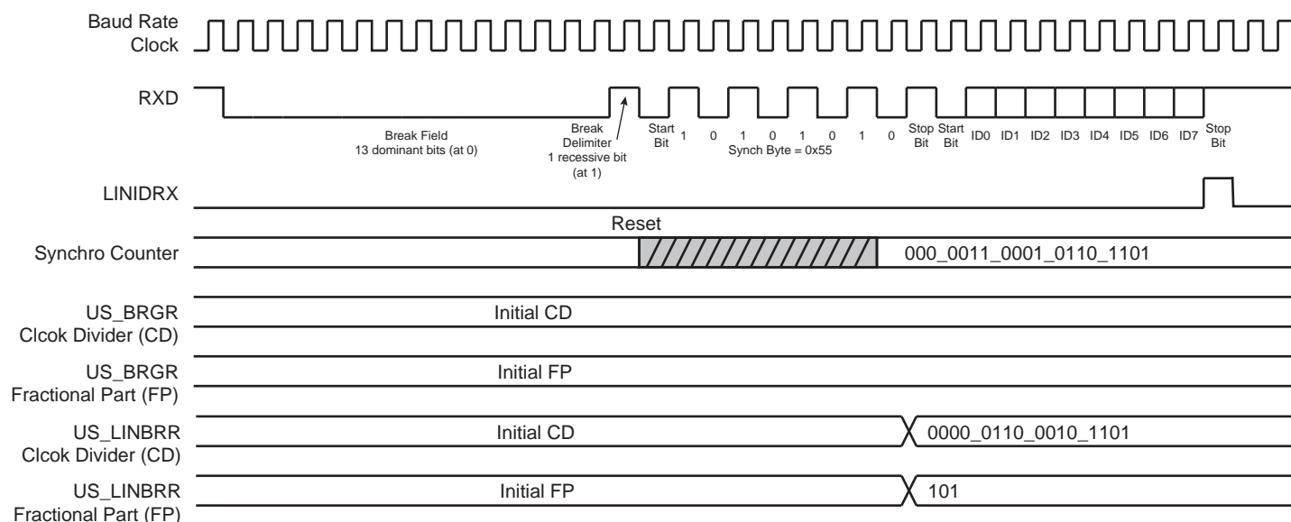
Figure 30-35. Slave Node Synchronization
