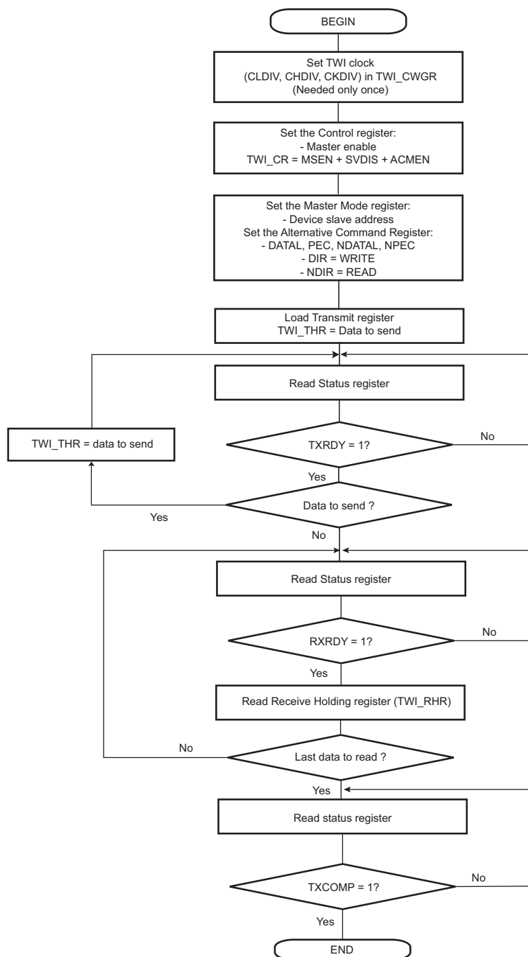
Figure 32-22. TWI Write Operation with Multiple Data Bytes + Read Operation and Alternative Command Mode + PEC
