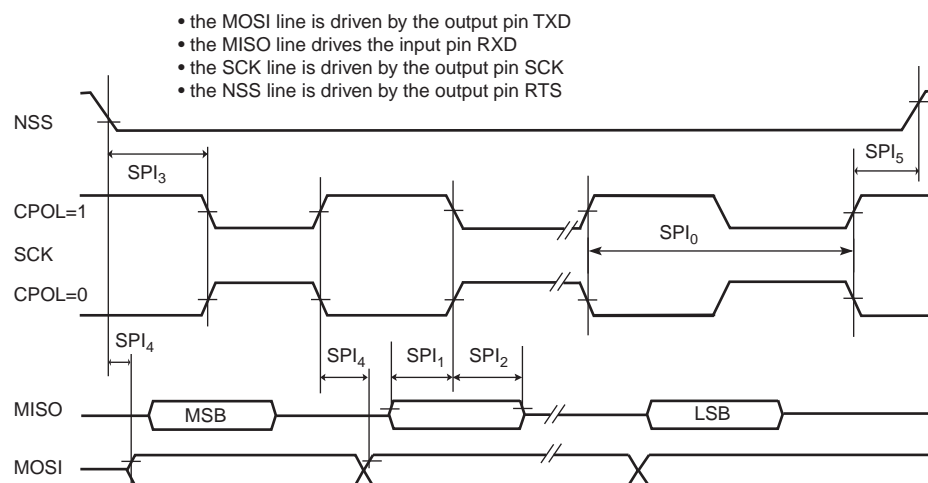
Figure 39-16. USART SPI Master Mode
