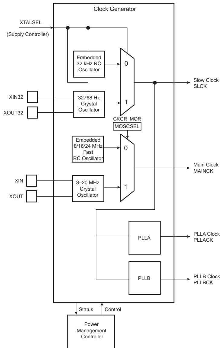
Figure 17-1. Clock Generator Block Diagram
