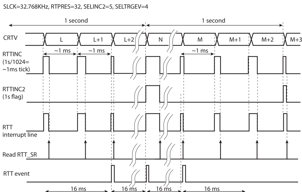
Figure 27-3. RTTINC2 behavior
