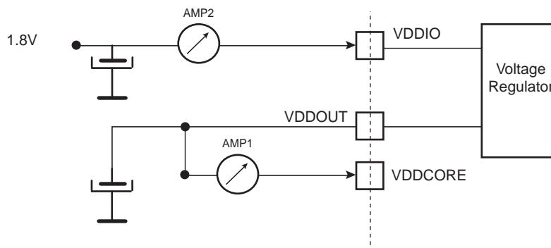
Figure 39-6. Measurement Setup for Sleep Mode
