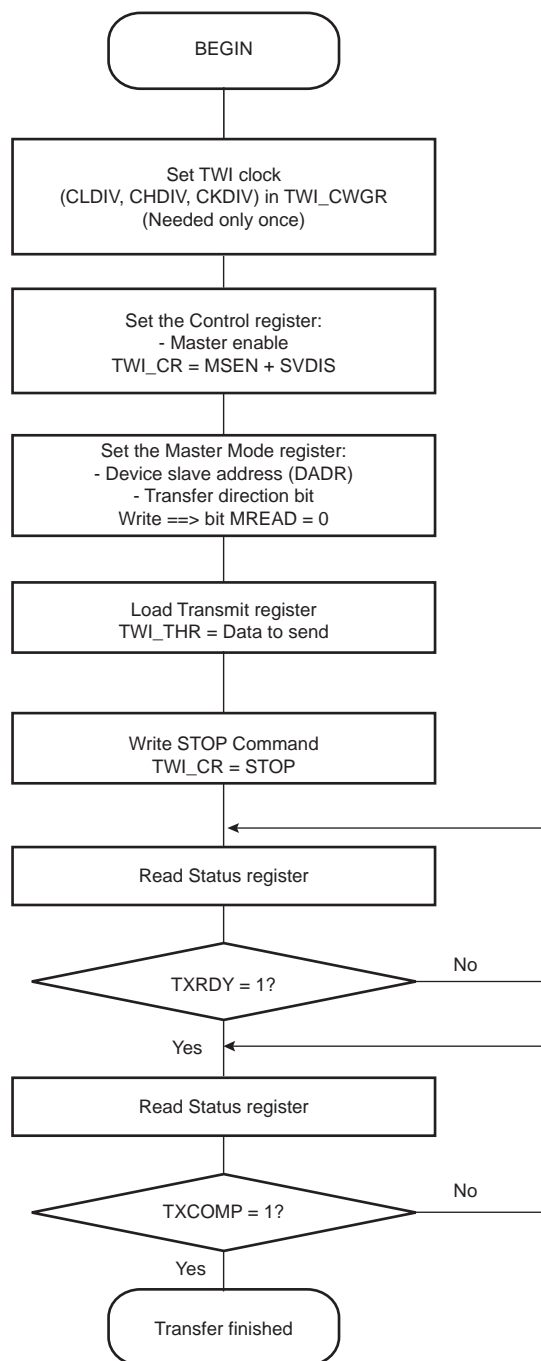
Figure 32-16. TWI Write Operation with Single Data Byte without Internal Address
