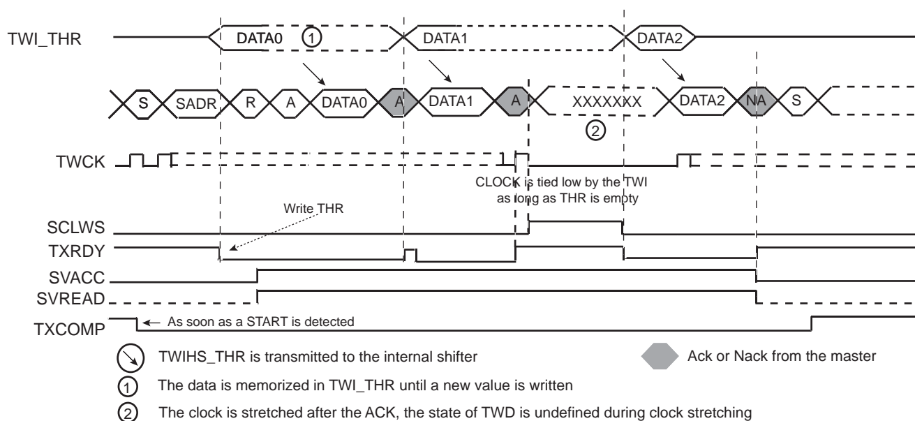
Figure 32-38. Clock Stretching in Read Mode
