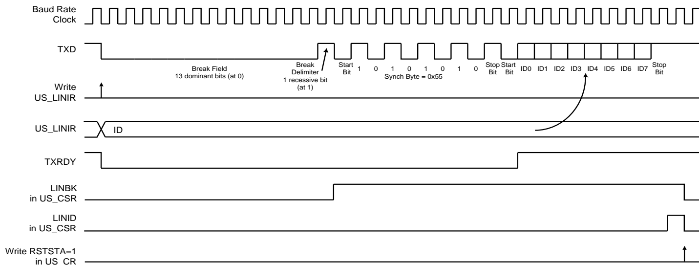
Figure 30-32. Header Transmission
