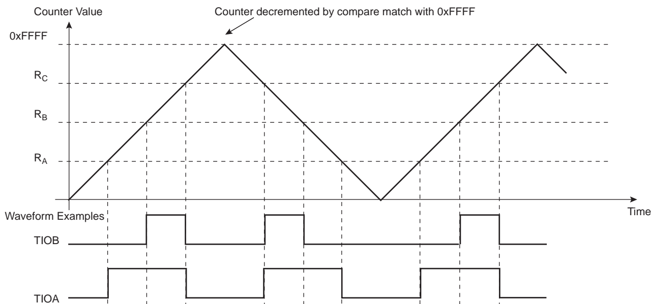
Figure 24-12. WAVSEL = 01 without Trigger
