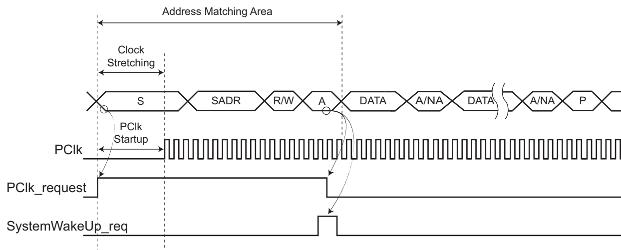
Figure 32-43. Address Match Only (Data Matching Disabled)
