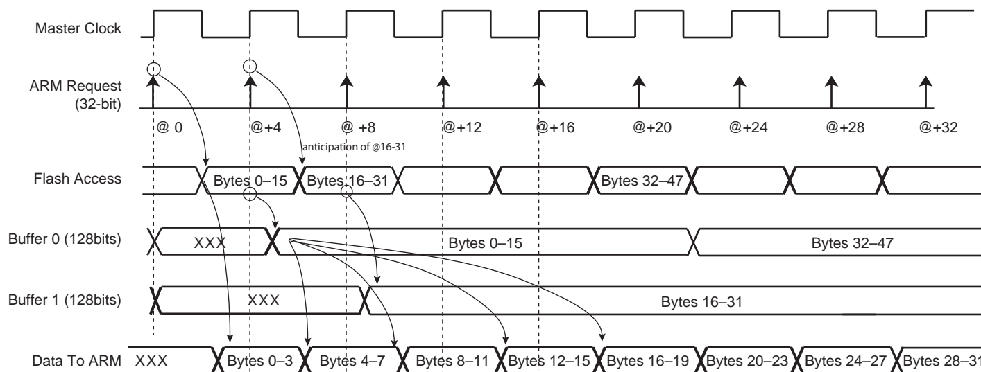
Figure 23-2. Code Read Optimization for FWS = 0
