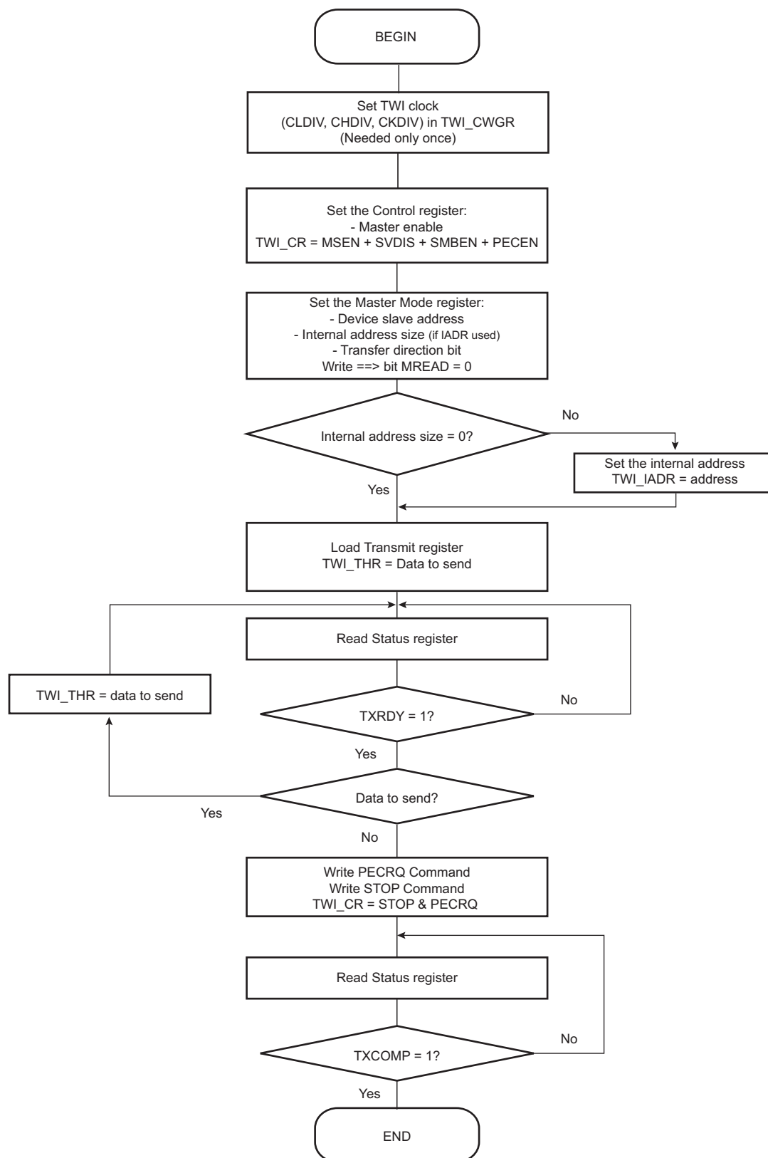
Figure 32-19. SMBus Write Operation with Multiple Data Bytes with or without Internal Address and PEC Sending
