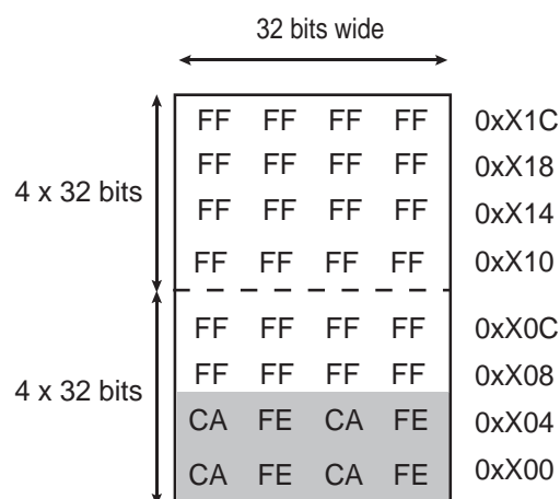
Figure 23-9. Optimized Partial Page Programming
