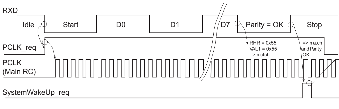
Figure 30-28. Asynchronous Wake-up Use Case Examples
