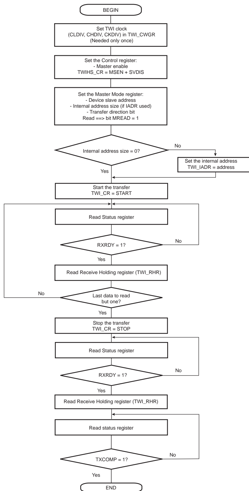
Figure 32-25. TWI Read Operation with Multiple Data Bytes with or without Internal Address
