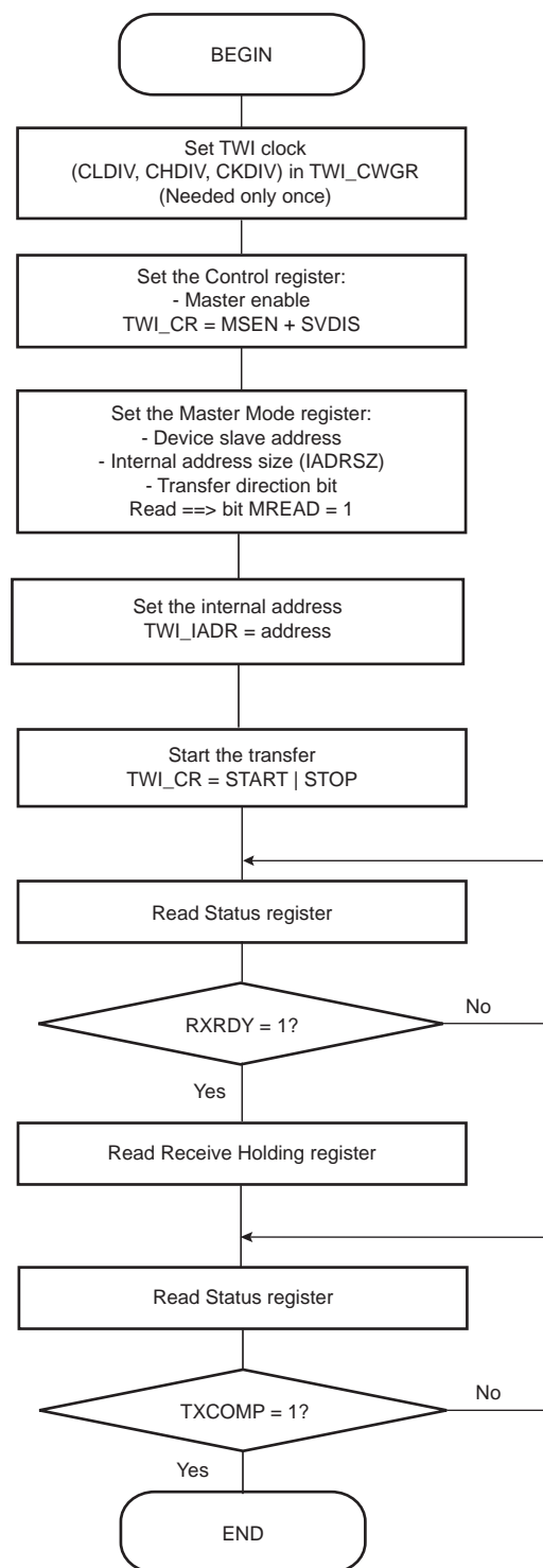
Figure 32-24. TWI Read Operation with Single Data Byte and Internal Address
