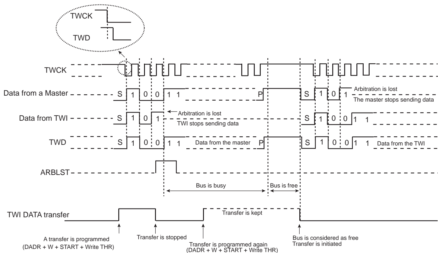
Figure 32-31. Arbitration Cases
