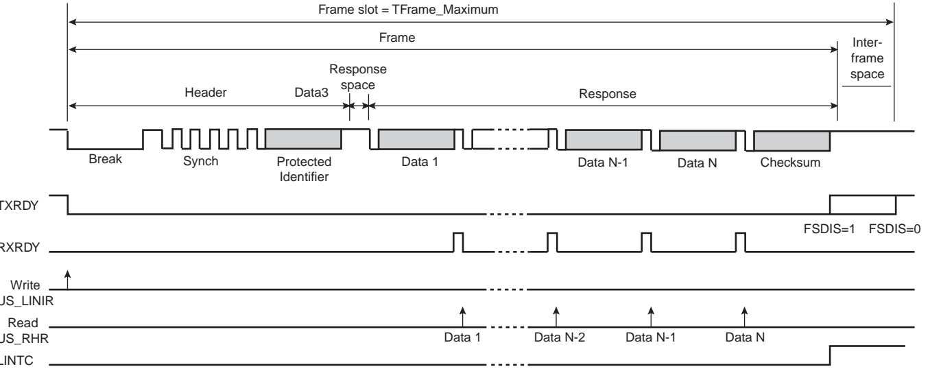
Figure 30-39. Master Node Configuration, NACT = SUBSCRIBE
