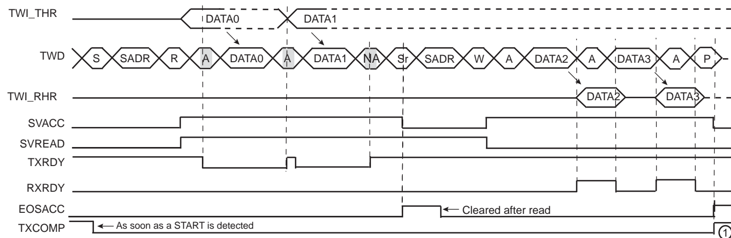
Figure 32-40. Repeated Start and Reversal from Read Mode to Write Mode
