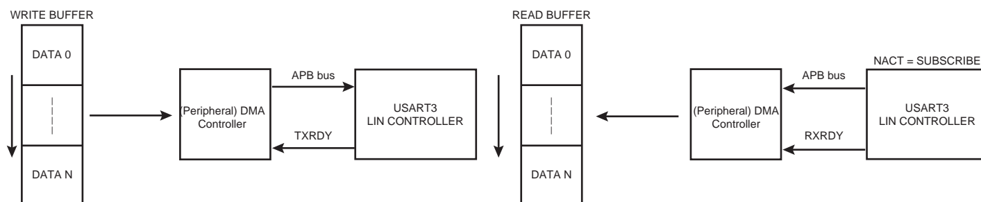
Figure 30-46. Slave Node with PDC
