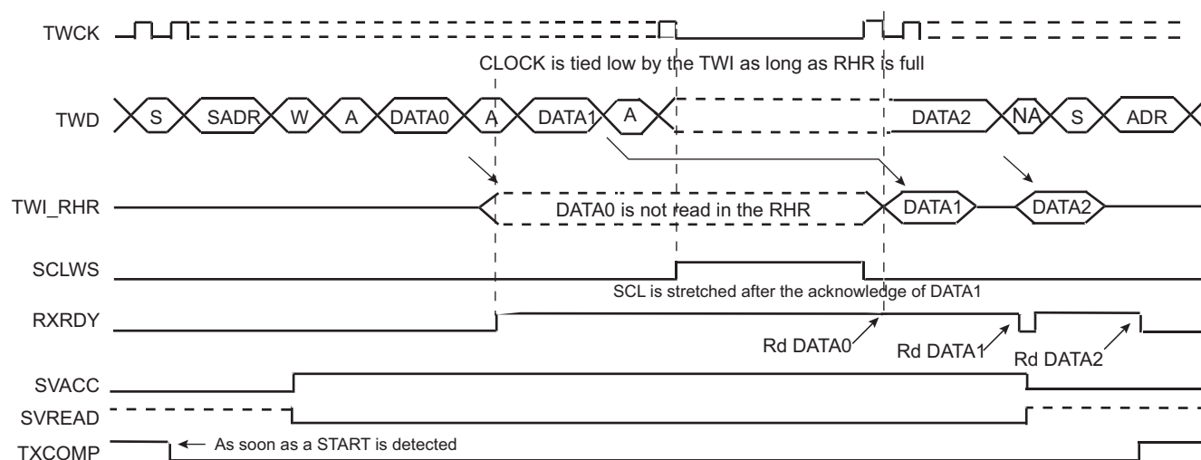
Figure 32-39. Clock Stretching in Write Mode
