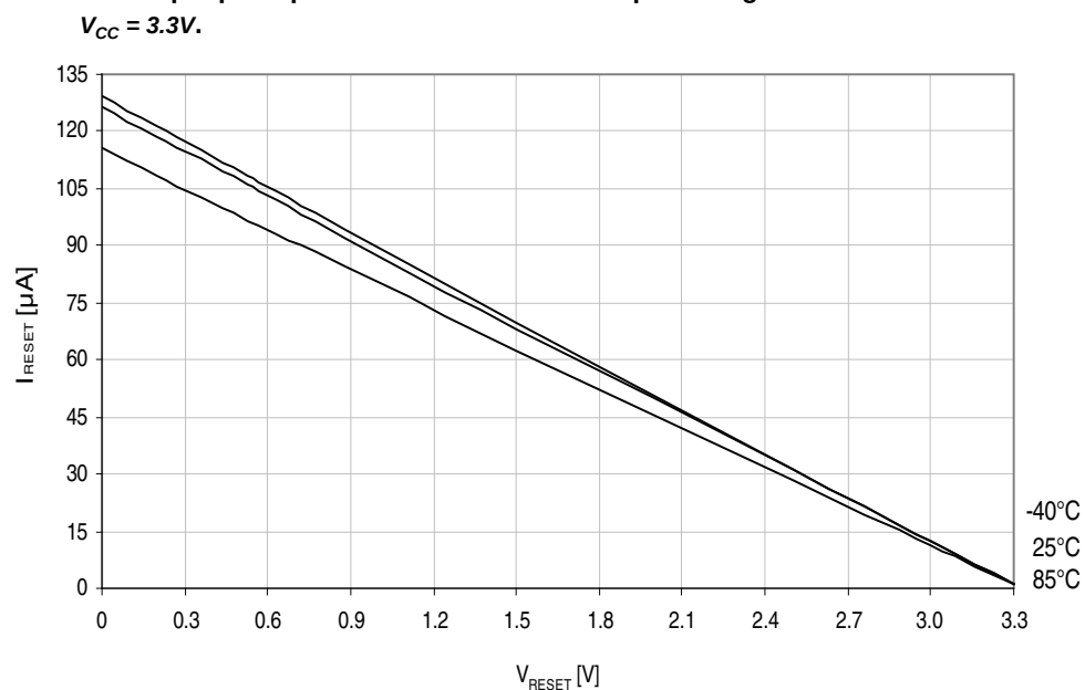
Figure 37-65. Reset pin pull-up resistor current vs. reset pin voltage.
