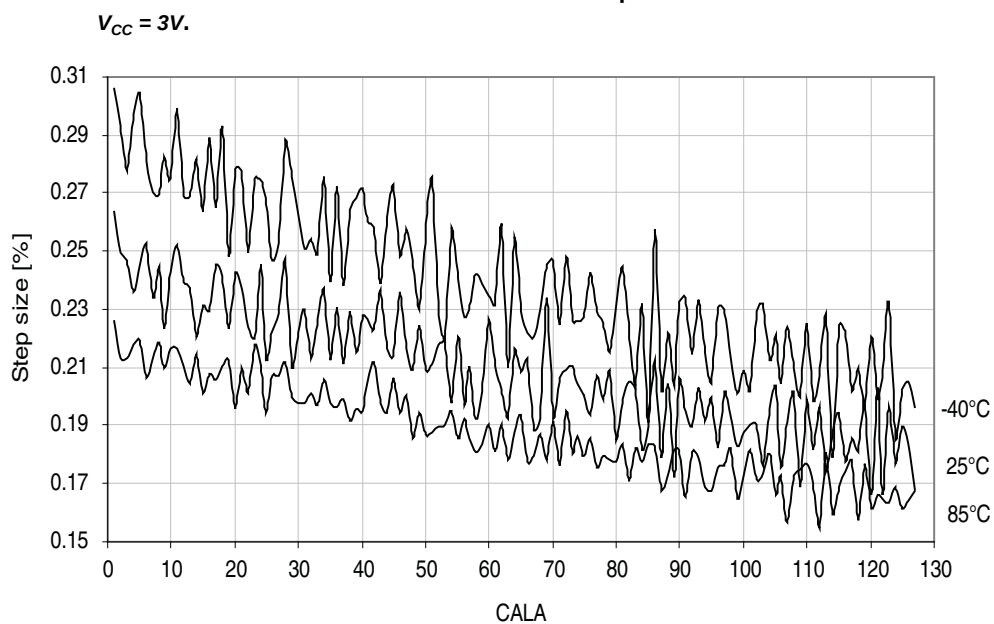
Figure 37-75. 2MHz internal oscillator CALA calibration step size.
