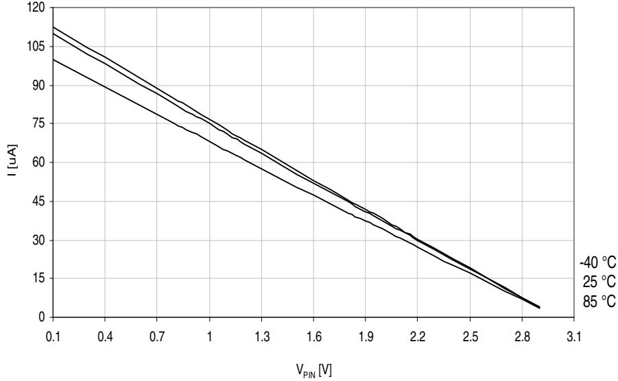
Figure 37-22. I/O pin pull-up resistor current vs. input voltage. V_{CC} = 3.0V .
