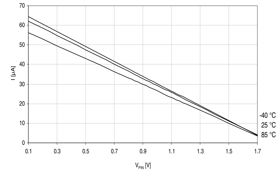
Figure 37-21. I/O pin pull-up resistor current vs. input voltage. V_{CC} = 1.8V .
