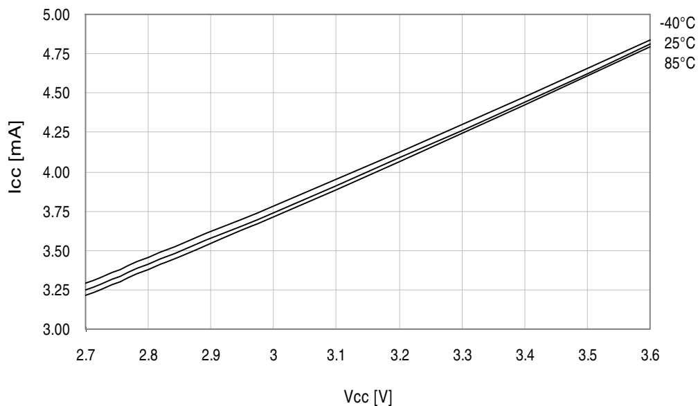
Figure 37-269. Idle mode current vs. V_{CC} .
