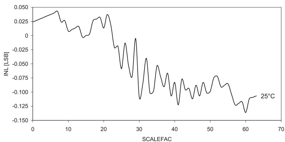
Figure 37-313. Voltage scaler INL vs. SCALEFAC.
