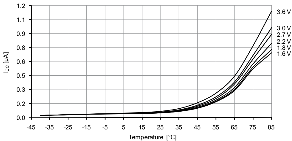
Figure 37-100. Power-down mode supply current vs. temperature. All functions disabled.
