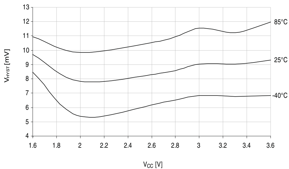
Figure 37-307. Analog comparator hysteresis vs. V_{CC} .
