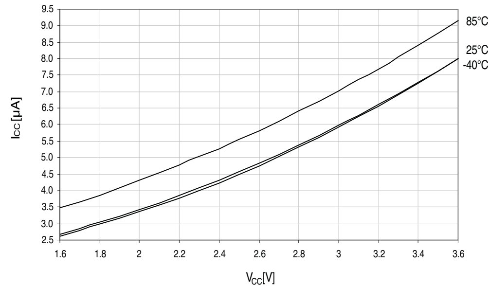
Figure 37-274. Standby supply current vs. V_{CC} . Standby, f_{SYS} = 1\text{MHz} .
