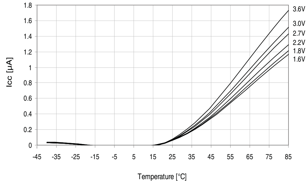
Figure 37-270. Power-down mode supply current vs. temperature. All functions disabled.
