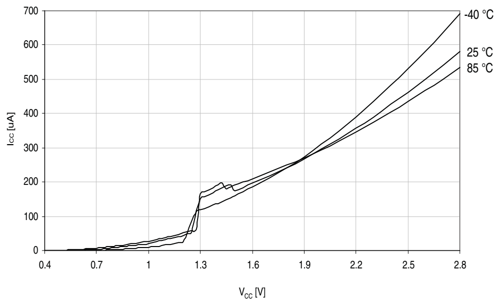
Figure 37-323. Power-on reset current consumption vs. V_{CC} .
