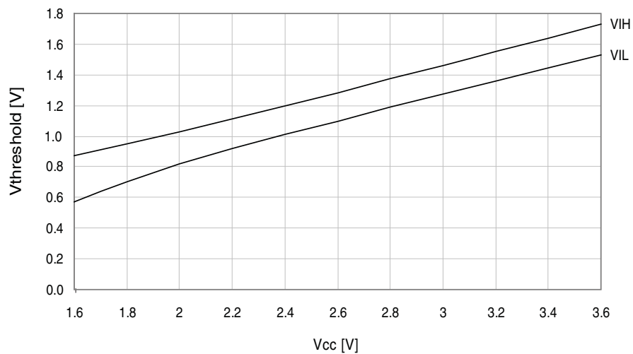
Figure 37-202. I/O pin input threshold voltage vs. V_{CC} .
