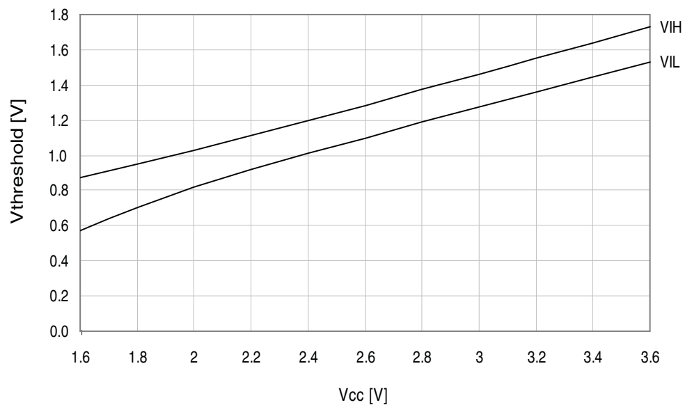
Figure 37-117. I/O pin input threshold voltage vs. V_{CC} . T = 25^{\circ}\text{C} .
