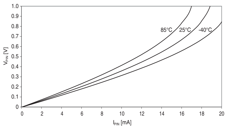
Figure 37-28. I/O pin output voltage vs. sink current.
