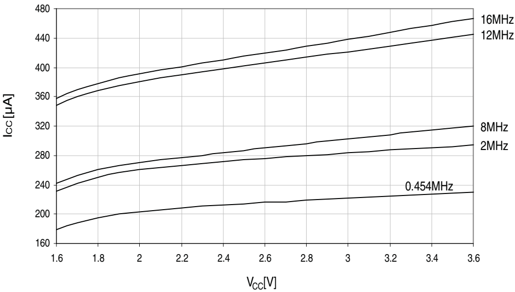
Figure 37-275. Standby supply current vs. V_{CC} . 25°C, running from different crystal oscillators.
