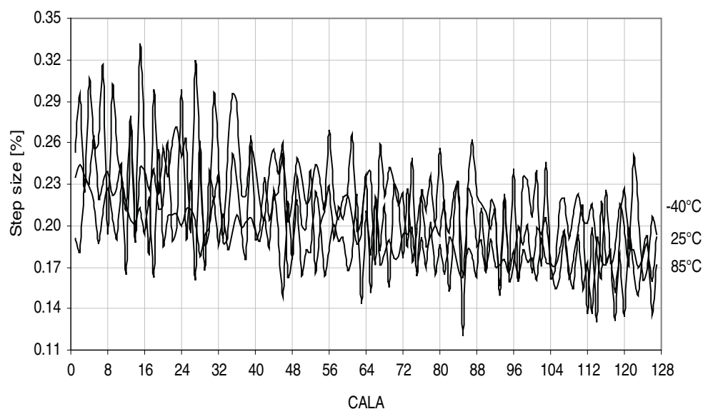
Figure 37-167. 48MHz internal oscillator CALA calibration step size. V CC = 3.0V.
