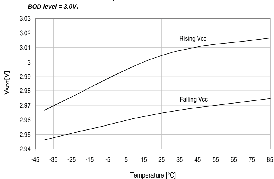
Figure 37-316. BOD thresholds vs. temperature.
