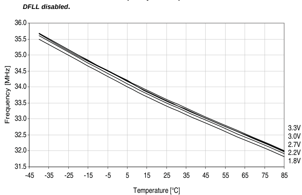
Figure 37-76. 32MHz internal oscillator frequency vs. temperature.
