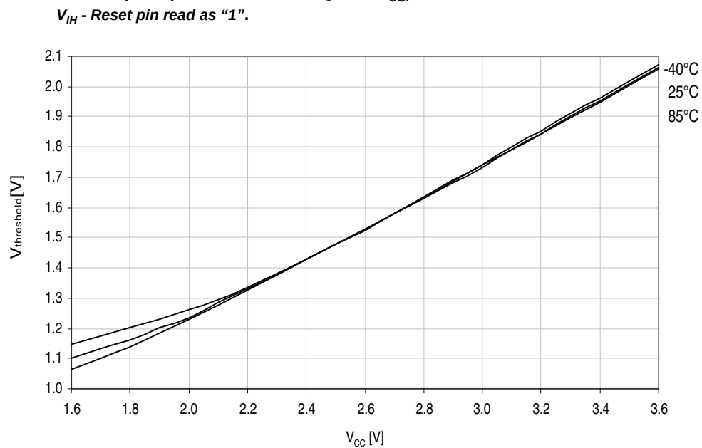
Figure 37-151. Reset pin input threshold voltage vs. V_{CC} .
