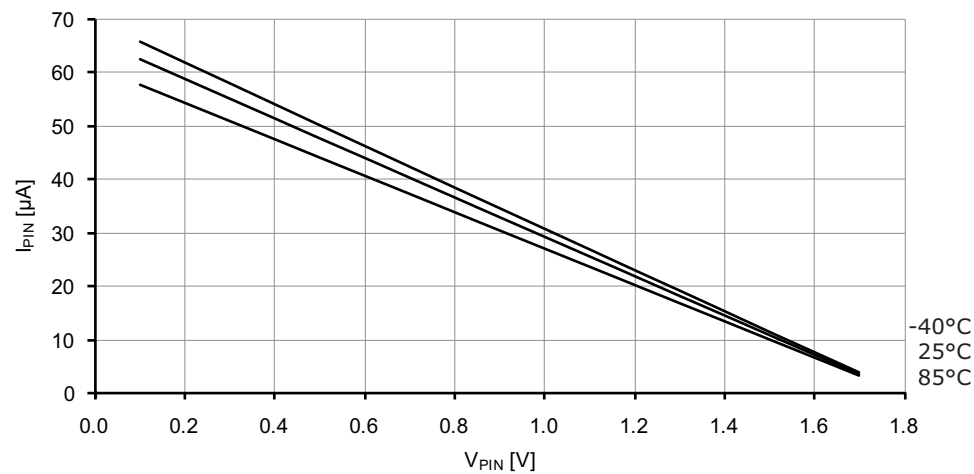
Figure 37-106. I/O pin pull-up resistor current vs. input voltage. V_{CC} = 1.8V .
