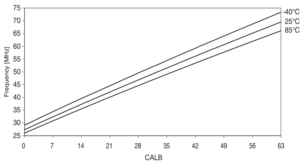
Figure 37-164. 32MHz internal oscillator frequency vs. CALB calibration value.
