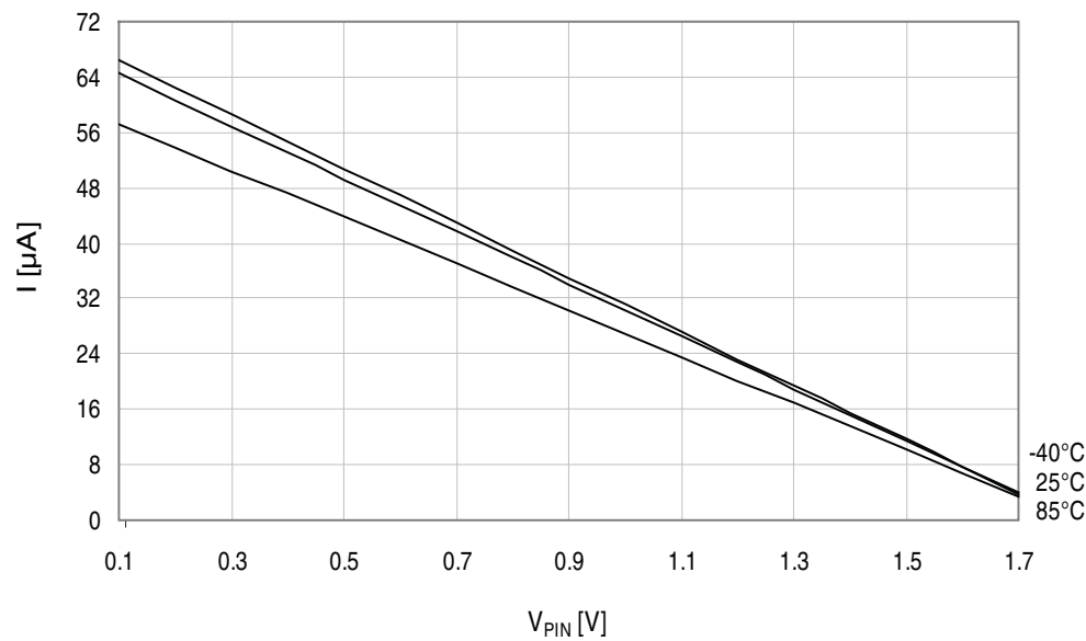
Figure 37-277. I/O pin pull-up resistor current vs. input voltage. V_{CC} = 3.0V .
