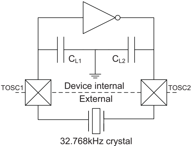
Figure 36-25.TOSC input capacitance.
