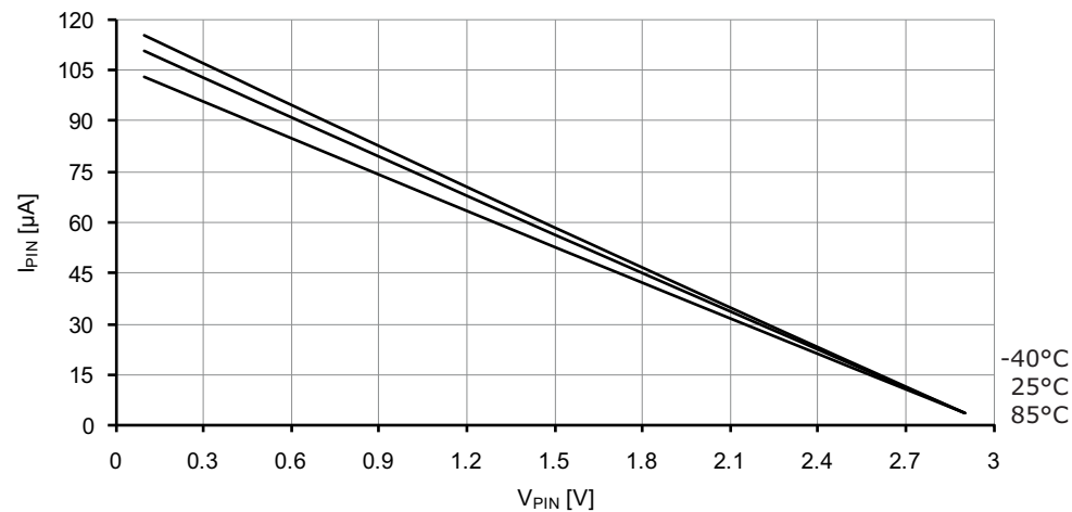
Figure 37-107. I/O pin pull-up resistor current vs. input voltage. V_{CC} = 3.0V .
