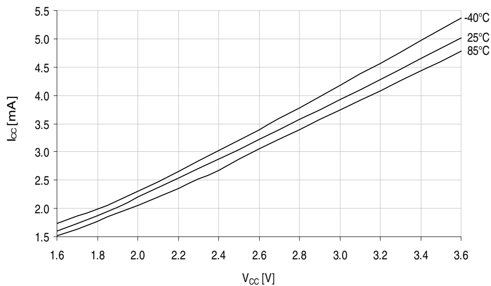
Figure 37-6. Active mode supply current vs. V_{CC} .
