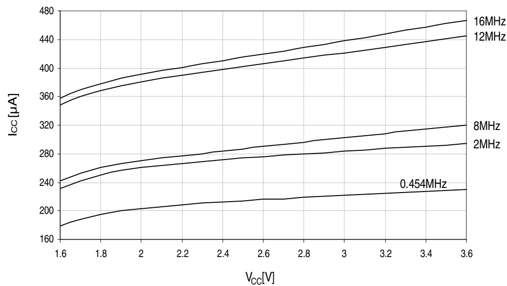
Figure 37-105. Standby supply current vs. V_{CC} . 25°C, running from different crystal oscillators.
