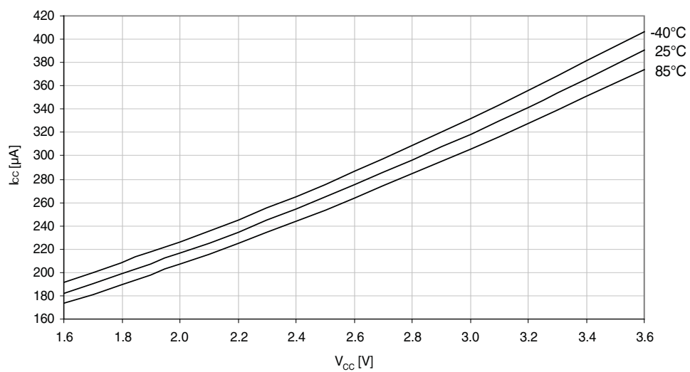
Figure 37-12. Idle mode supply current vs. V_{CC} .
