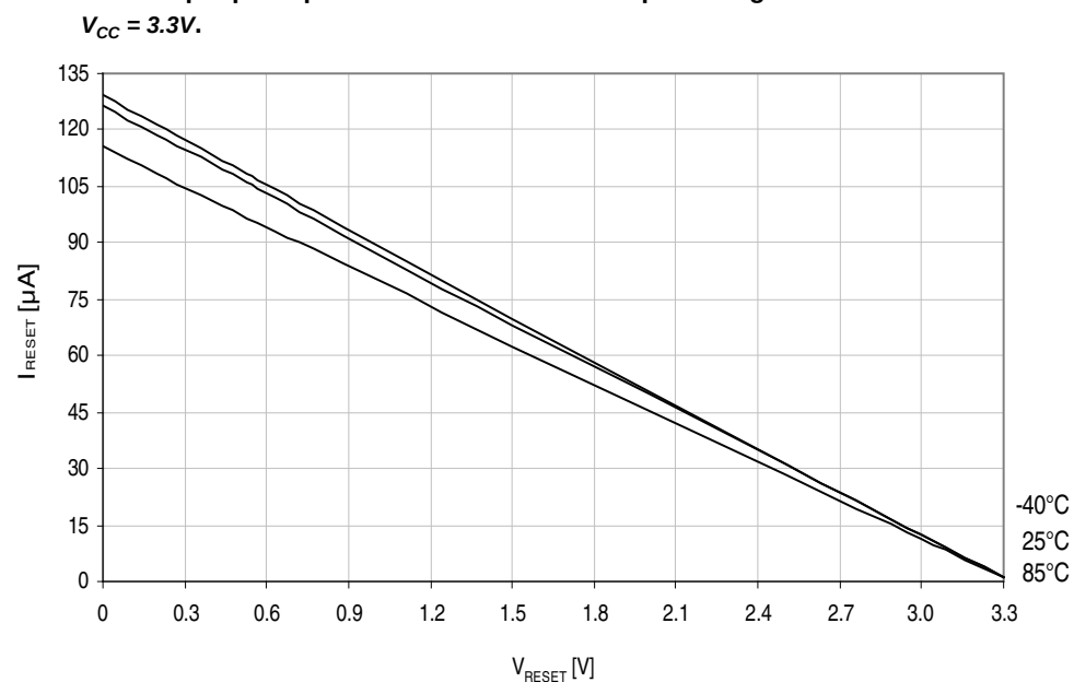
Figure 37-150. Reset pin pull-up resistor current vs. reset pin voltage.
