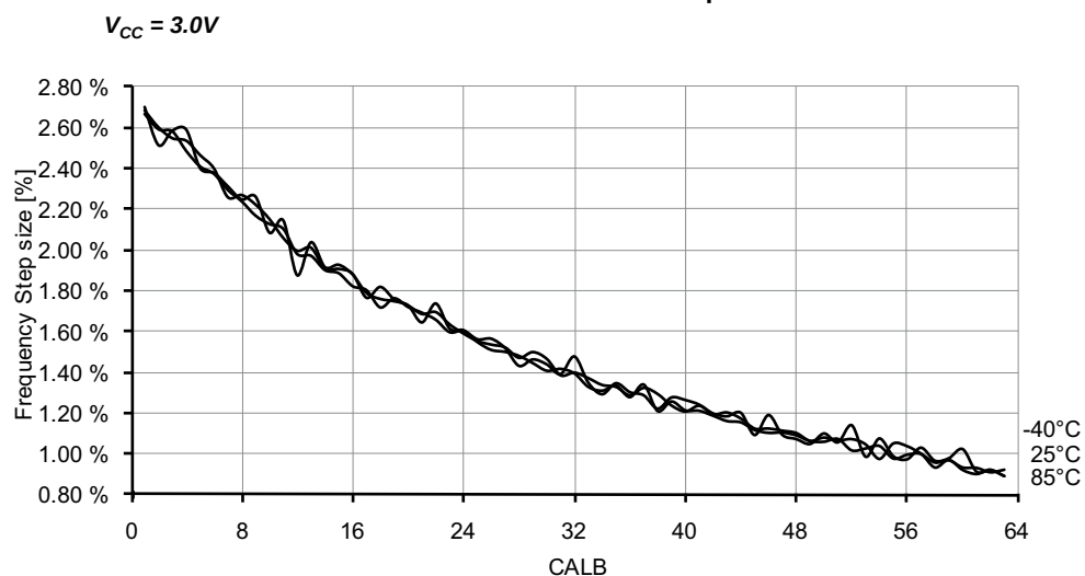
Figure 37-249. 32MHz internal oscillator CALB calibration step size.
