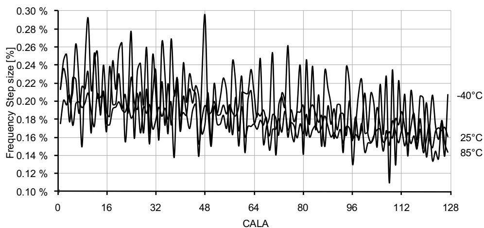
Figure 37-252. 48MHz internal oscillator CALA calibration step size. V_{CC} = 3.0V
