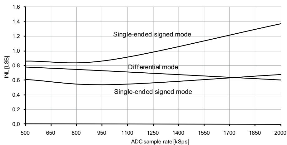
Figure 37-207. INL error vs. sample rate. T = 25^{\circ}\text{C} , V_{CC} = 2.7\text{V} , V_{REF} = 1.0\text{V external} .
