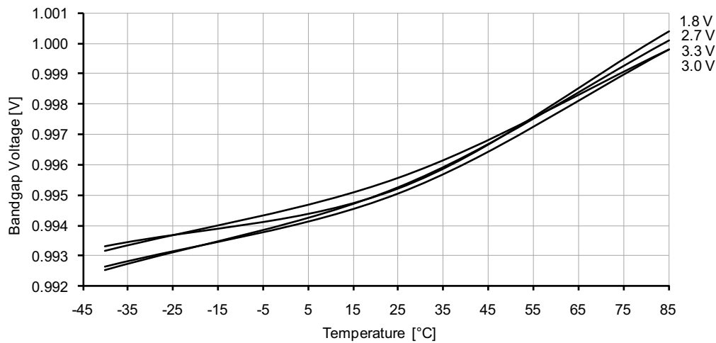
Figure 37-229. ADC/DAC Internal 1.0V reference vs. temperature.
