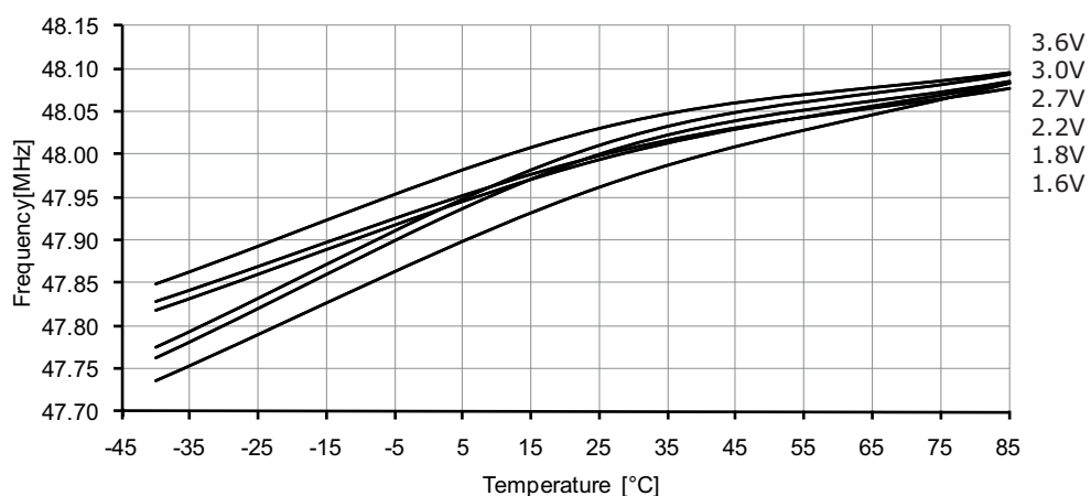
Figure 37-251. 48MHz internal oscillator frequency vs. temperature. DPLL enabled, from the 32.768kHz internal oscillator.
