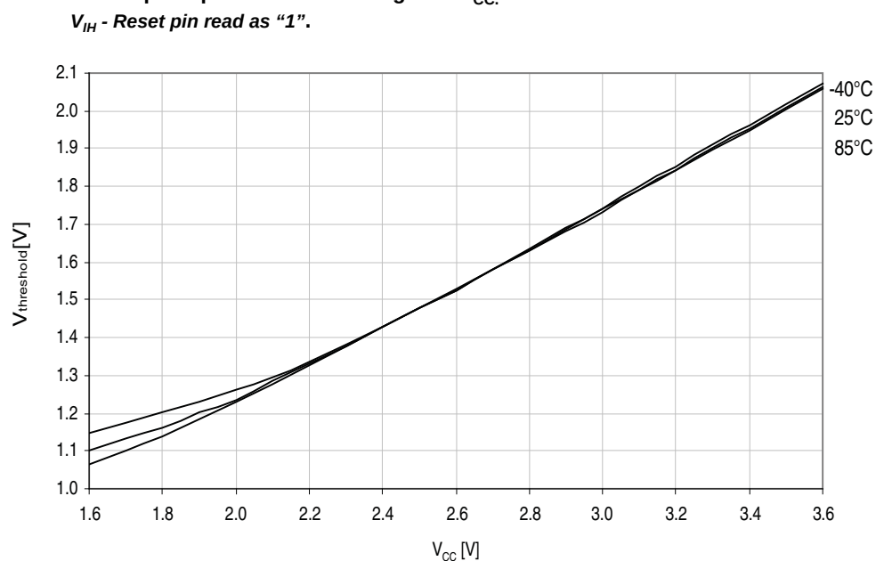
Figure 37-66. Reset pin input threshold voltage vs. V_{CC} .
