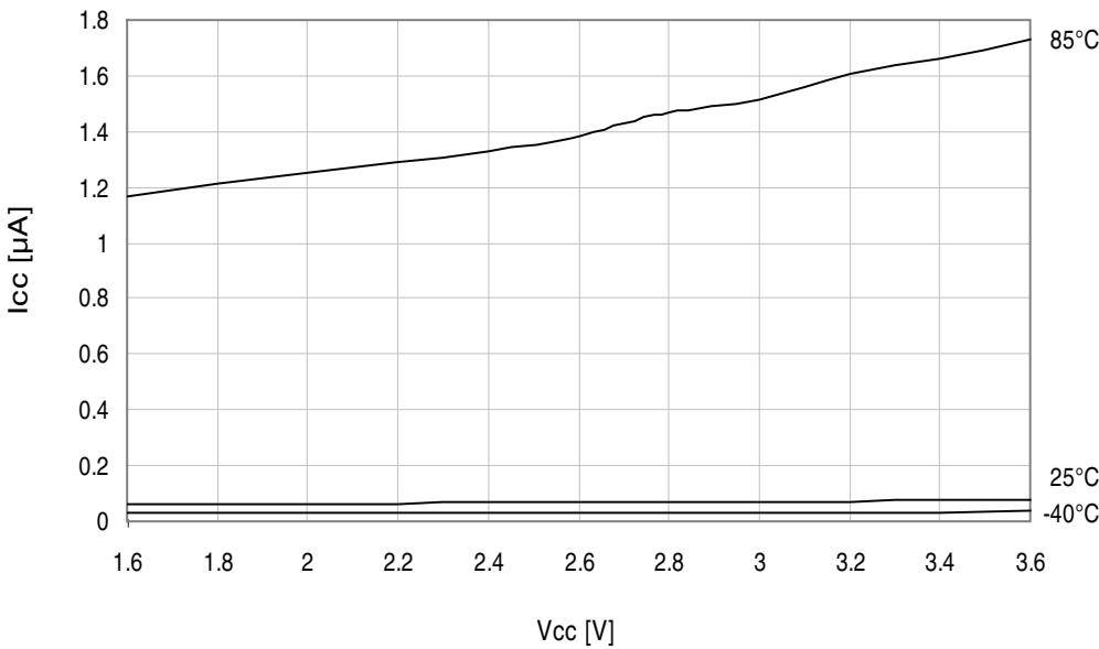
Figure 37-271. Power-down mode supply current vs. V_{CC} . All functions disabled.
