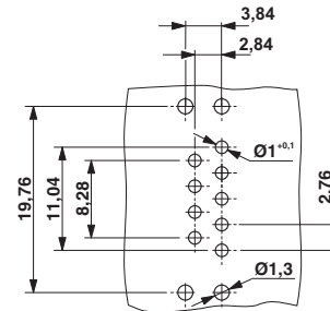
Drilling diagram
