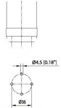
Direct Mounting
