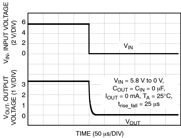
Figure 25. Turn-Off
