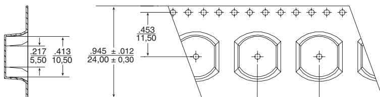
TAPE & REEL LAYOUT
