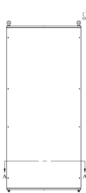
REAR VIEW
