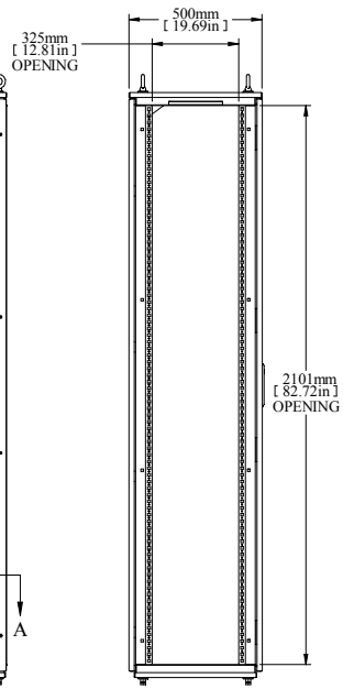
L.S. VIEW
