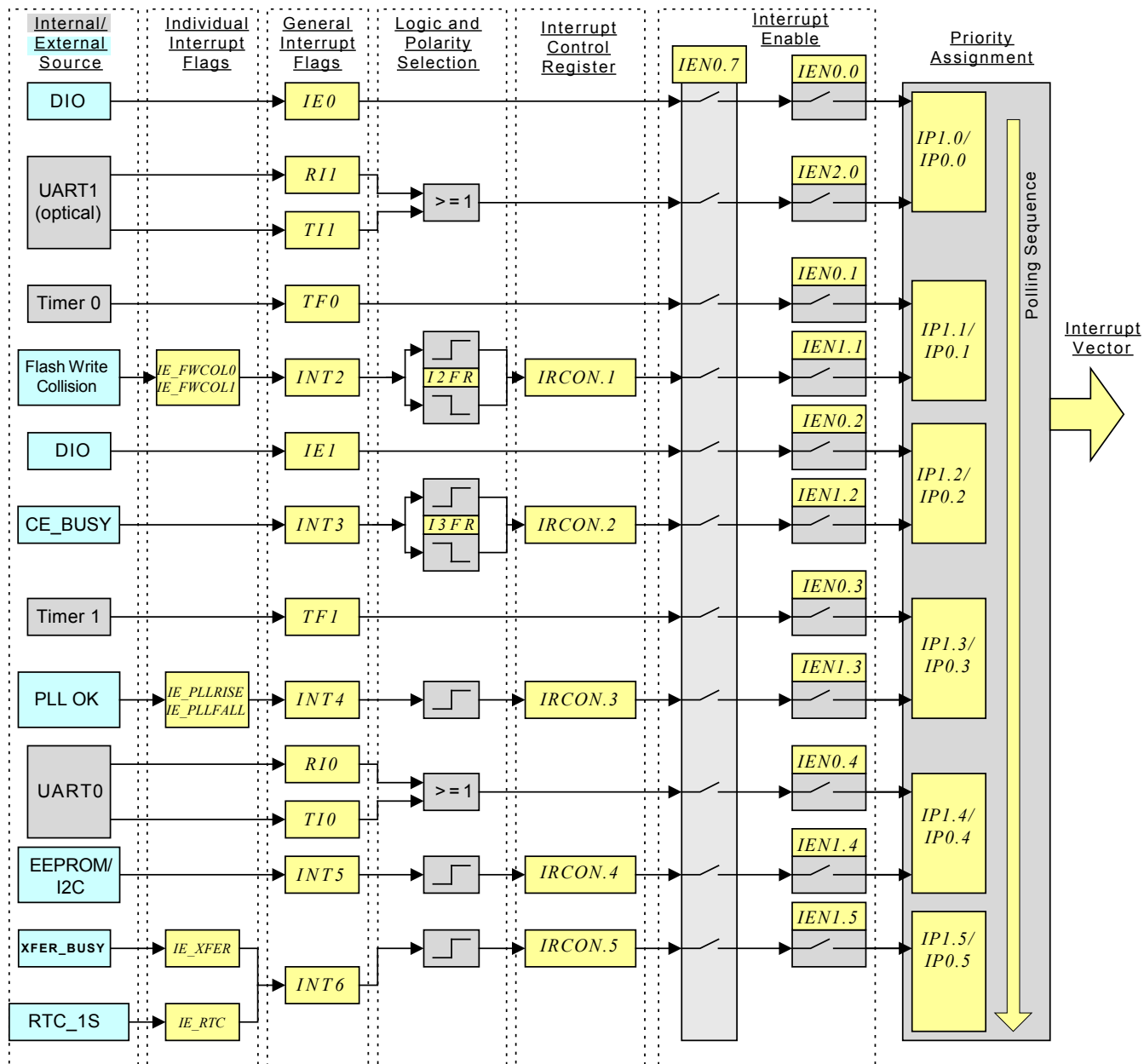
Figure 6: Interrupt Structure
