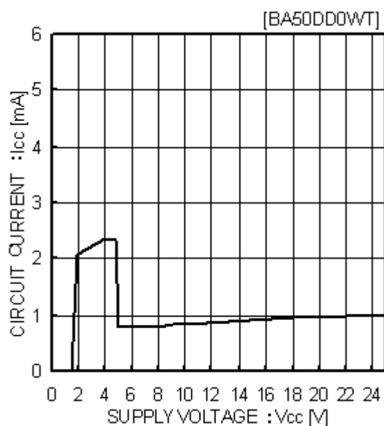
Fig.15 Circuit Current
