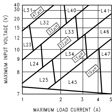
Figure 19. LM2679-5.0
