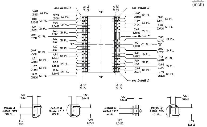
BOTTOM VIEW
