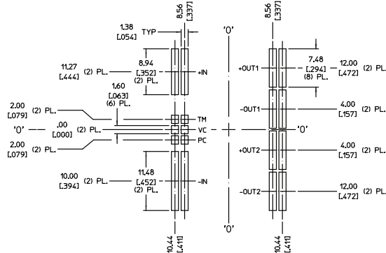
RECOMMENDED LAND PATTERN (COMPONENT SIDE SHOWN)
