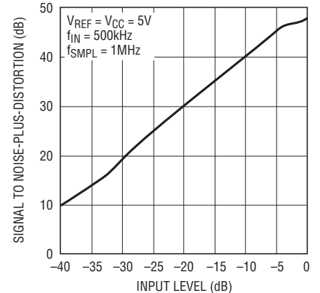
S/(N + D) vs Input Level
