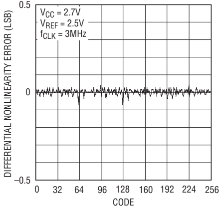
Differential Nonlinearity vs Code at 2.7V
