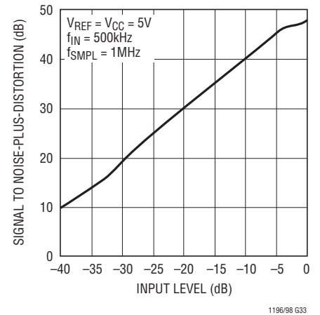
S/(N + D) vs Input Level
