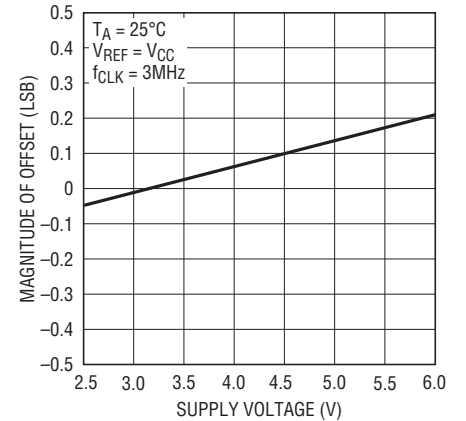
Offset vs Supply Voltage
