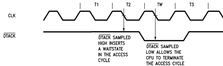
FIGURE 21. \overline{\text{DTACK}} Type Output
