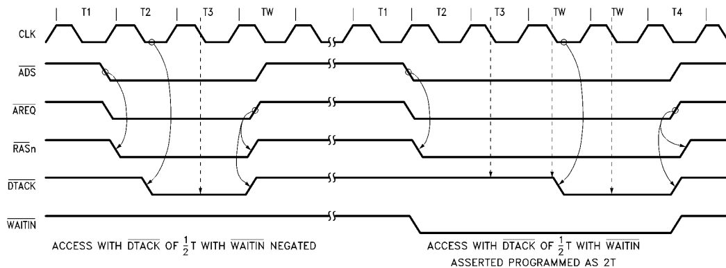
FIGURE 22a. \overline{\text{WAITIN}} Example ( \overline{\text{DTACK}} is Sampled at the "T3" Falling Clock Edge)
