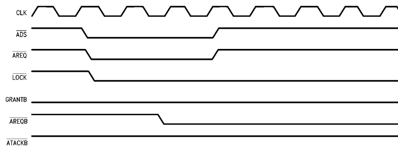
FIGURE 33. \overline{\text{LOCK}} Function
